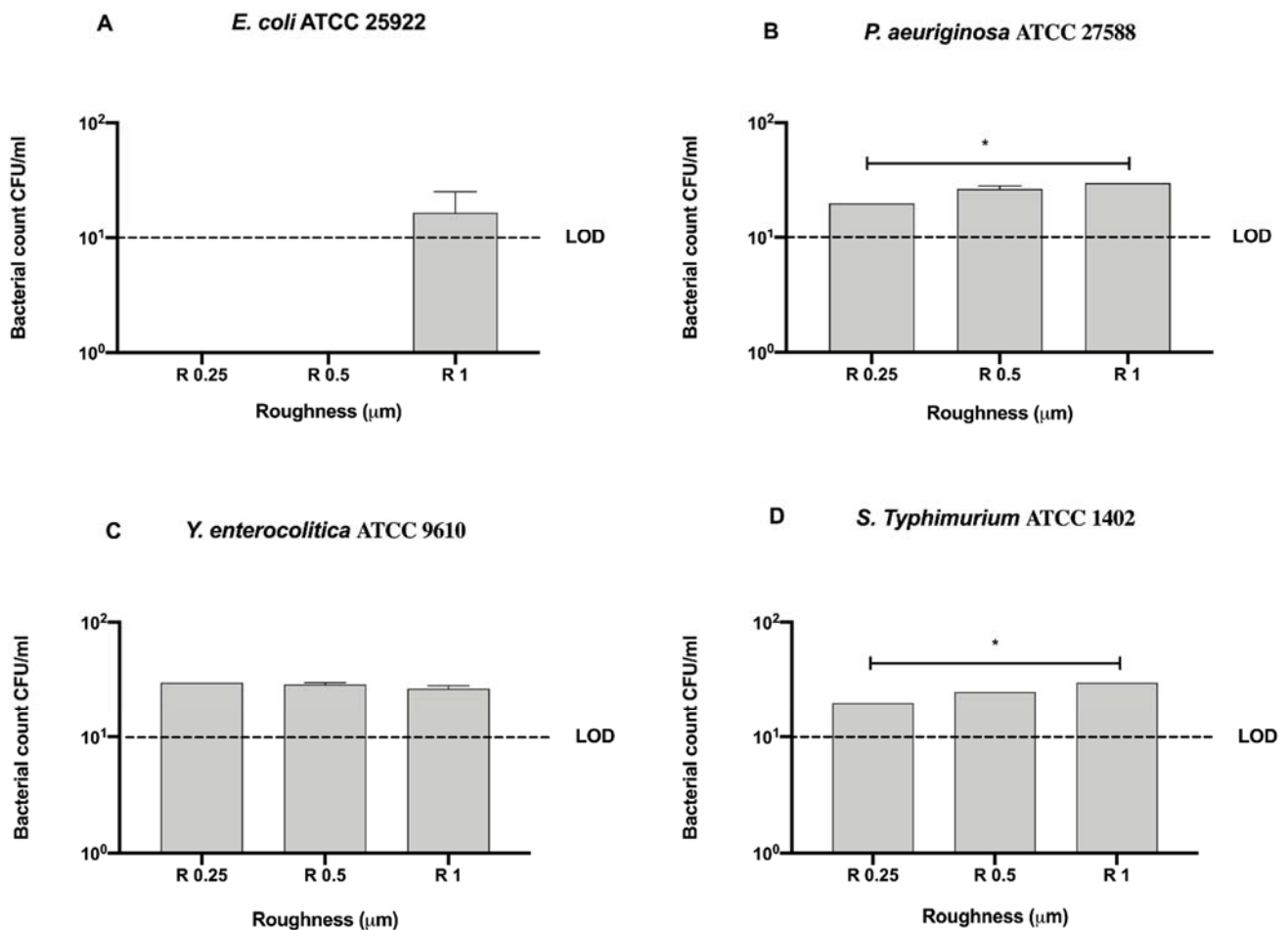
Figure 8. Graphical representation of the antibacterial activity of different AISI 316 stainless steel surface roughness coated with nanoXHAM® D against Gram-negative bacteria (A–D), * p < 0.05 ; Limit of detection (LOD) is 10^1 ( 10E+1 ).
