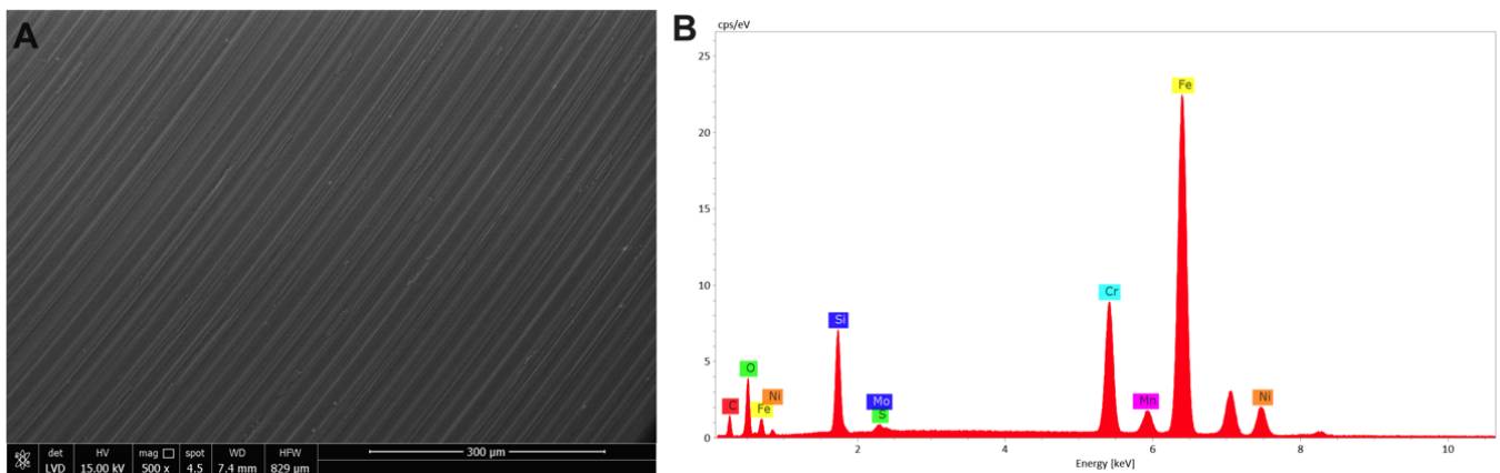
Figure 12. Environmental scanning microscopy morphological analysis on a (A) nanoXHAM® D-treated stainless steel disk surface observed at 300 µm along with its (B) X-EDS microanalysis.
