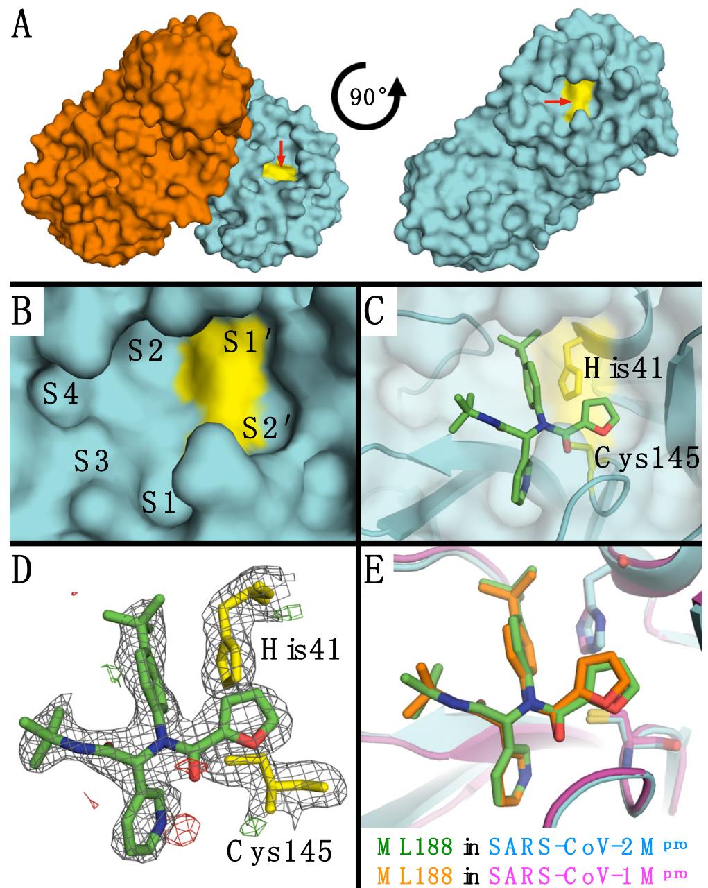
Figure 2. (A) SARS2-M PRO dimer and single subunit shown in surface representation (rotated on the plane of the page). (B) SARS2-M PRO active site with subsites labeled and catalytic residues colored yellow. (C) ML188 in the SARS2-M PRO active site with catalytic residues labeled. (D) Electron density around ML188 and catalytic residues. The 2F_o - F_c direct maps are depicted as grey mesh contoured at 1.0 \sigma while the F_o - F_c difference maps have positive density depicted as green mesh contoured at 3.0 \sigma and negative density as red mesh contoured at -3.0 \sigma . (E) Alignment of ML188 in SARS2-M PRO (teal protein and green ligand; PDB: 7L0D) and SARS1-M PRO (magenta protein and orange ligand; PDB: 3V3M).
