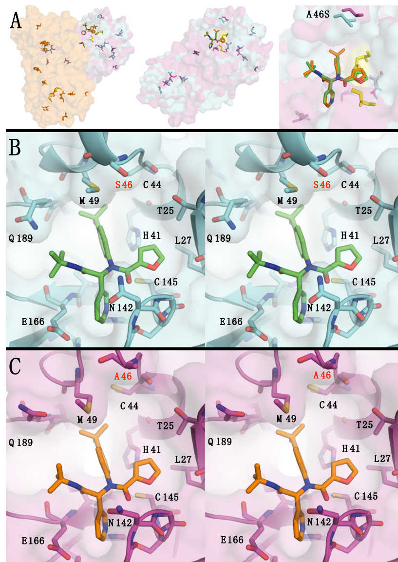
Figure 3. (A) The twelve amino acid differences between SARS2 and SARS1-MP PRO shown as a dimer, single subunit, and active site. SARS2 (in cyan) and SARS1 (in magenta) are shown with transparent surfaces and amino acid differences shown as sticks. The dimer subunits (in orange) and the catalytic residues (in yellow) are included. (B) Stereo pair of SARS2-MP PRO -ML188 complex active site. (C) Stereo pair of SARS1-MP PRO -ML188 complex active site.
