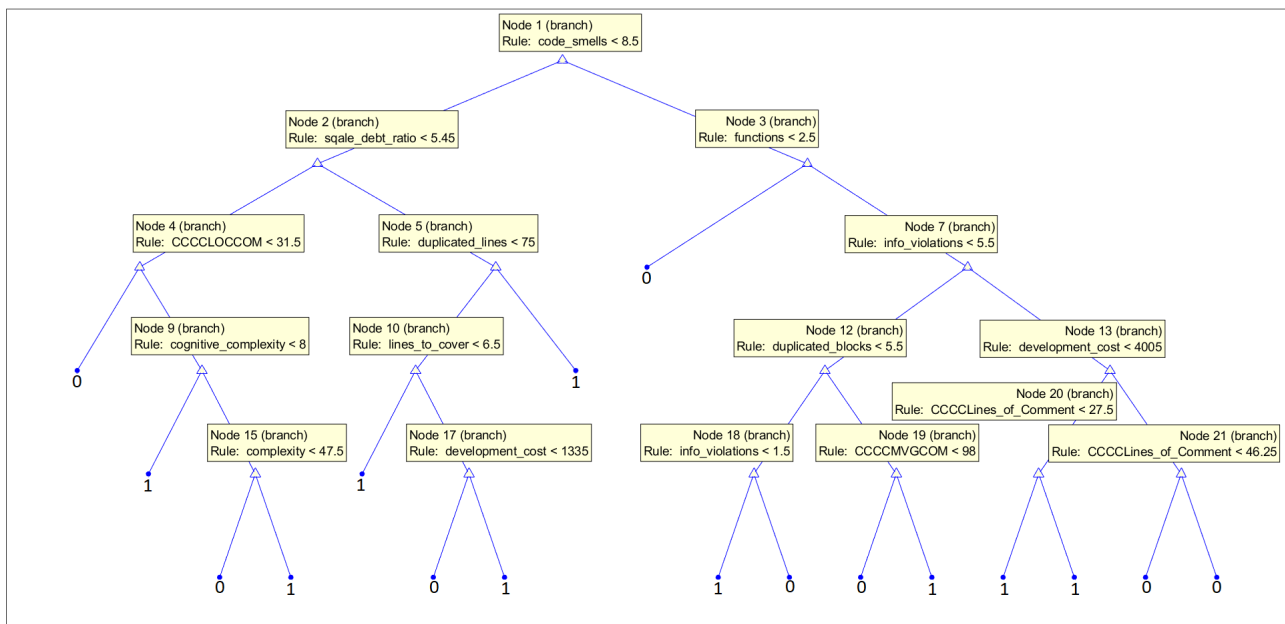
Figure 17. Medium tree based given all 33 features as an input for the subset with CWE-119 vulnerabilities considered.
