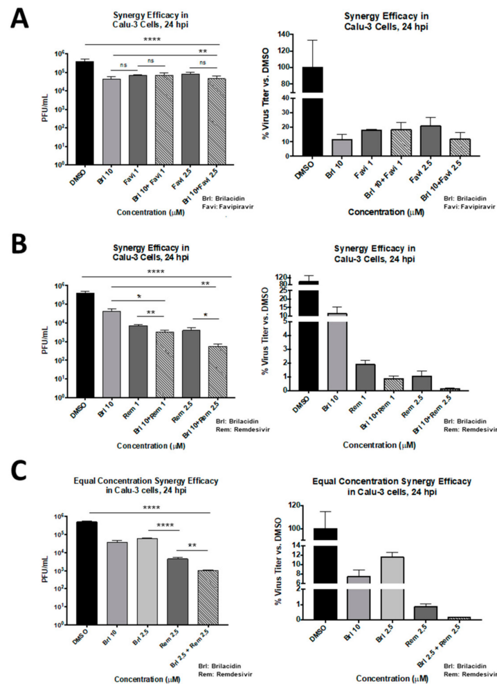
Figure 5. Efficacy of brilacidin as a combinatorial strategy as assessed in Calu-3 cells. Calu-3 cells were pretreated for 2 h with media alone or media containing brilacidin at 10 \mu\text{M} (for synergy treatments). (A) Cells were infected with SARS-CoV-2 at MOI 0.05 directly with brilacidin at 10 \mu\text{M} (for synergy treatments) or SARS-CoV-2 incubated in media alone (for favipiravir treatment alone). After 1 h, post-treatment with favipiravir alone or mixed with 10 \mu\text{M} brilacidin were added to cells at 1 or 2.5 \mu\text{M} concentrations. At 24 hpi, viral supernatants were evaluated by plaque assay as described in Materials and Methods. Calu-3 cells were pretreated for 2 h with media alone or media containing brilacidin at 10 or 2.5 \mu\text{M} (for synergy treatments). Cells were infected with SARS-CoV-2 at MOI 0.05 directly with brilacidin at 10 or 2.5 \mu\text{M} (for synergy treatments) or SARS-CoV-2 incubated in media alone (for remdesivir treatment alone). After 1 h, post-treatment with remdesivir alone, or mixed with 10 \mu\text{M} (B) or 2.5 \mu\text{M} (C) brilacidin, were added to cells at 1 or 2.5 \mu\text{M} concentrations. At 24 hpi, viral supernatants were evaluated by plaque assay as described in Materials and Methods. Graphs are representative of one independent experiment performed in technical triplicates ( n = 3 ). Brl indicates brilacidin, Rem indicates remdesivir. Statistical analyses for synergy vs. individual control treatments were determined using Unpaired Two-Tailed Student's t test. Significance against DMSO was determined as described in Materials and Methods. * p < 0.0332 , ** p < 0.0021 , **** p < 0.0001 .
