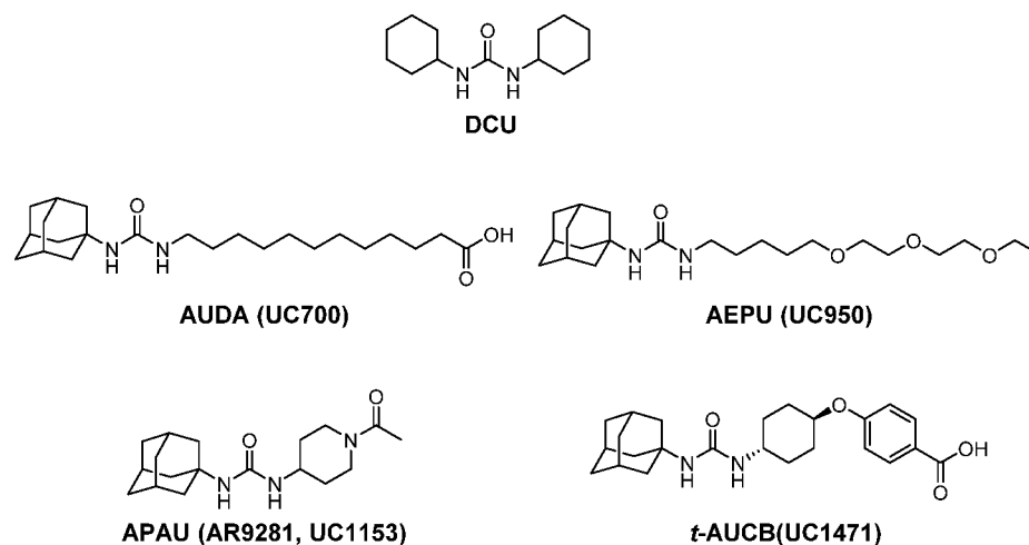
Figure 1. Chemical structures of early stage sEHI. A commonly used four-letter abbreviation and a University of California (UC) number are provided. Our lead compound in this series was DCU. The presence of an adamantyl group made the sEHI more potent and easier to detect by LC-MS in blood. They also tended to mimic EpFA, which were the presumptive substrates.
