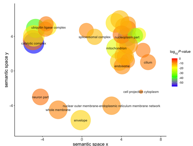
Figure 2. REVIGO visualization of GO cellular component terms significantly associated with mtDNA-CN after removal of redundant GO terms. Size of the circle represents the relative number of genes in each gene set, color represents significance. Axes represent semantic similarities between GO terms; GO terms that are more similar will cluster with one another.
