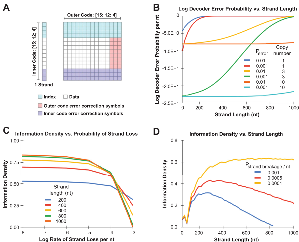
Fig. 2 Analysis of tradeoffs between system reliability, information density, strand length, and error rates. A Reed-Solomon inner-outer encoding scheme. B Relationship between log decoder error probability during RS decoding and DNA strand length, including the effects of symbol error rate (mutations, insertions, and deletion, P_{\text{error}} ) and copy number. C Relationship between information density of a DNA storage system and the probability of symbol erasure (strand loss due to breakage) as a function of strand length. D Relationship between information density and strand length as a function of the probability of strand breakage. C and D assume a copy number of 1.
