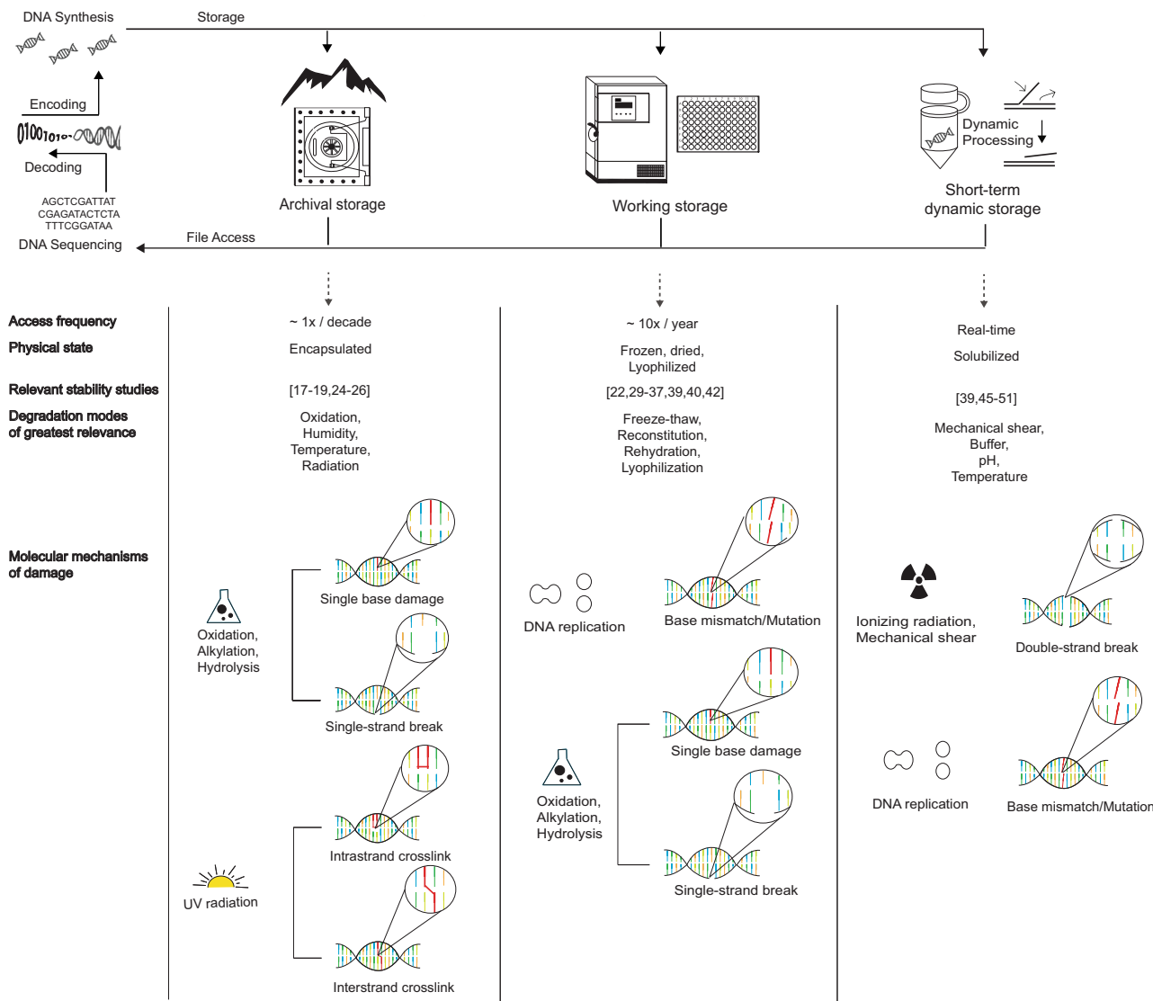
Fig. 1 Categories of DNA storage with distinct longevities, functional characteristics, and degradation modes. (Top) A generic DNA-based system showing distinct types of storage modes. (Middle) Functional and physical characteristics of each storage mode. (Bottom) Molecular mechanisms of damage most relevant to each storage mode.
