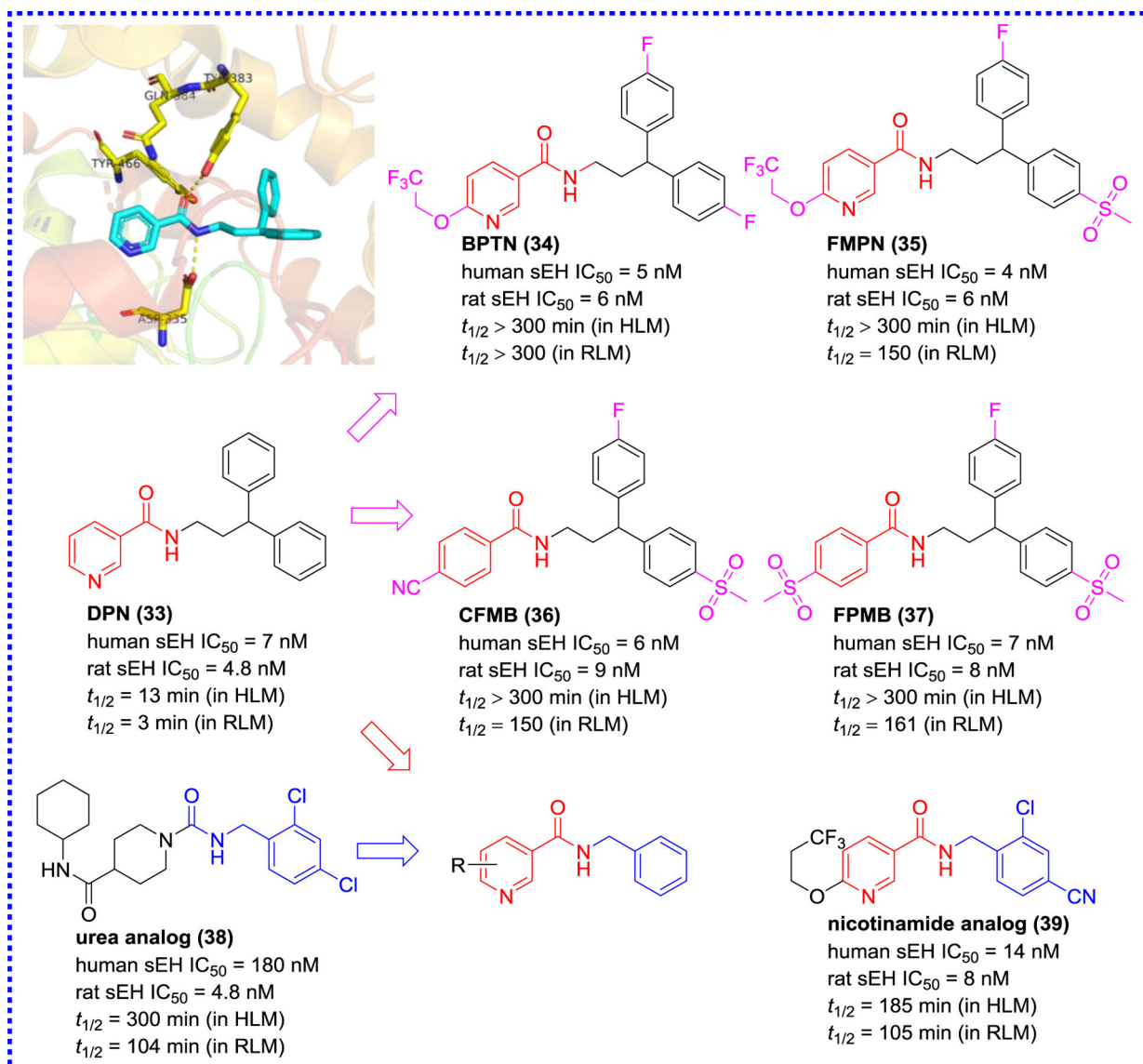
Figure 9. X-ray co-crystal structure of DPN (33) with sEH (PDB code 311Y) and its optimization.
