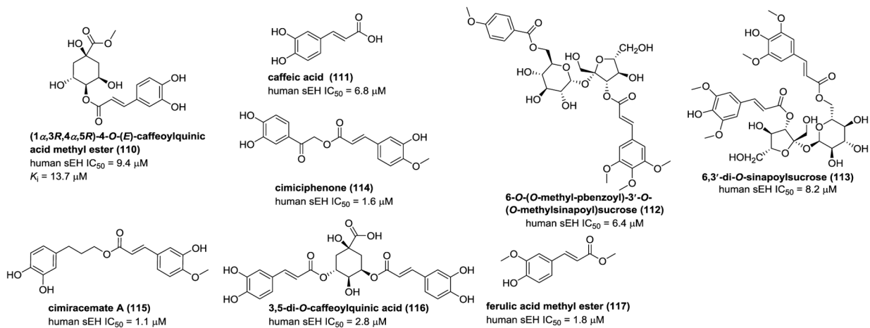
Figure 32. Chemical structures of naturally occurring sEH inhibitors: phenylpropionic acids (110–117).
