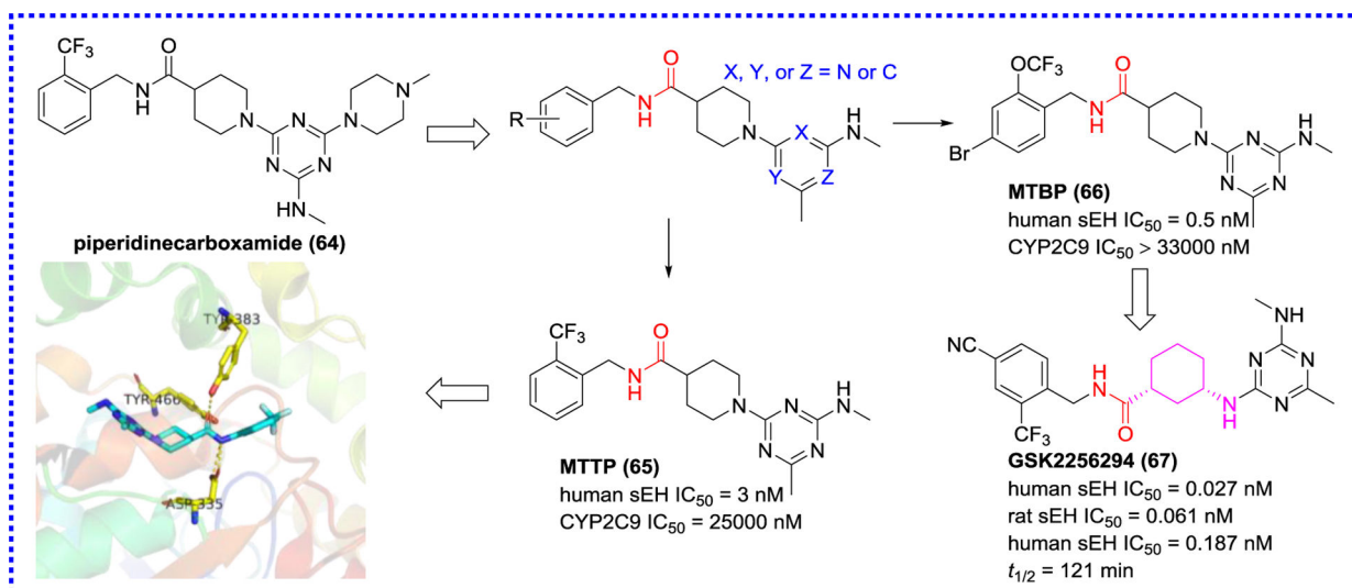
Figure 15. Modification based on the structure of the amide ( 64 ) and co-crystal structure of MTPP ( 65 ) and sEH (PDB code 4JNC)
