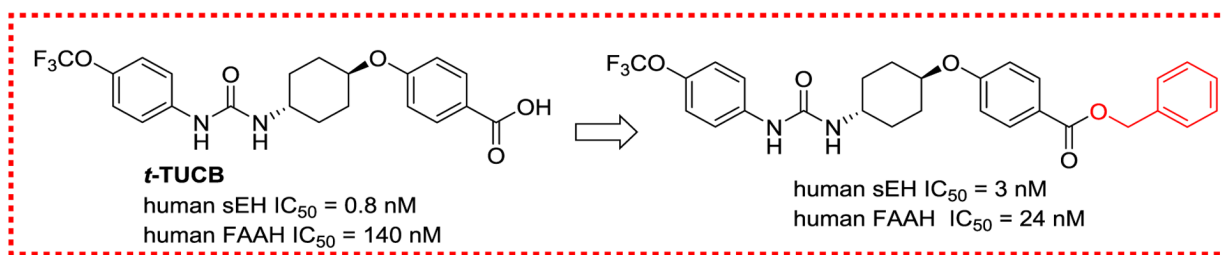
Figure 21. A sEH/FAAH dual inhibitor derived from t -TUCB.
