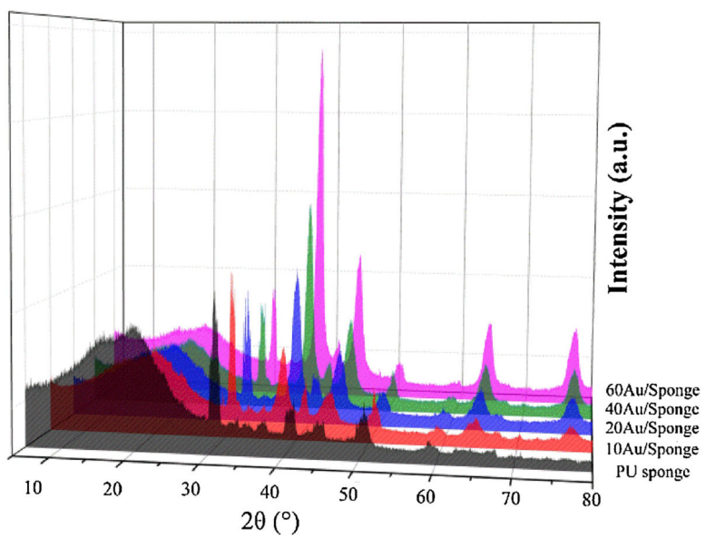
Fig.6. X-ray diffraction patterns of different catalyst samples.
