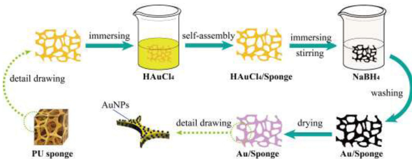
Scheme.1. Preparation of the AuNP/Sponge catalyst.
