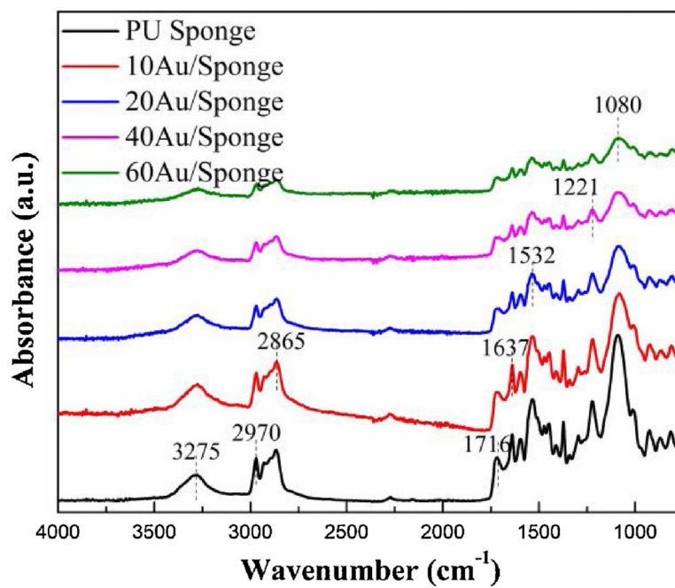
Fig.7. FT-IR spectra of different catalyst samples.
