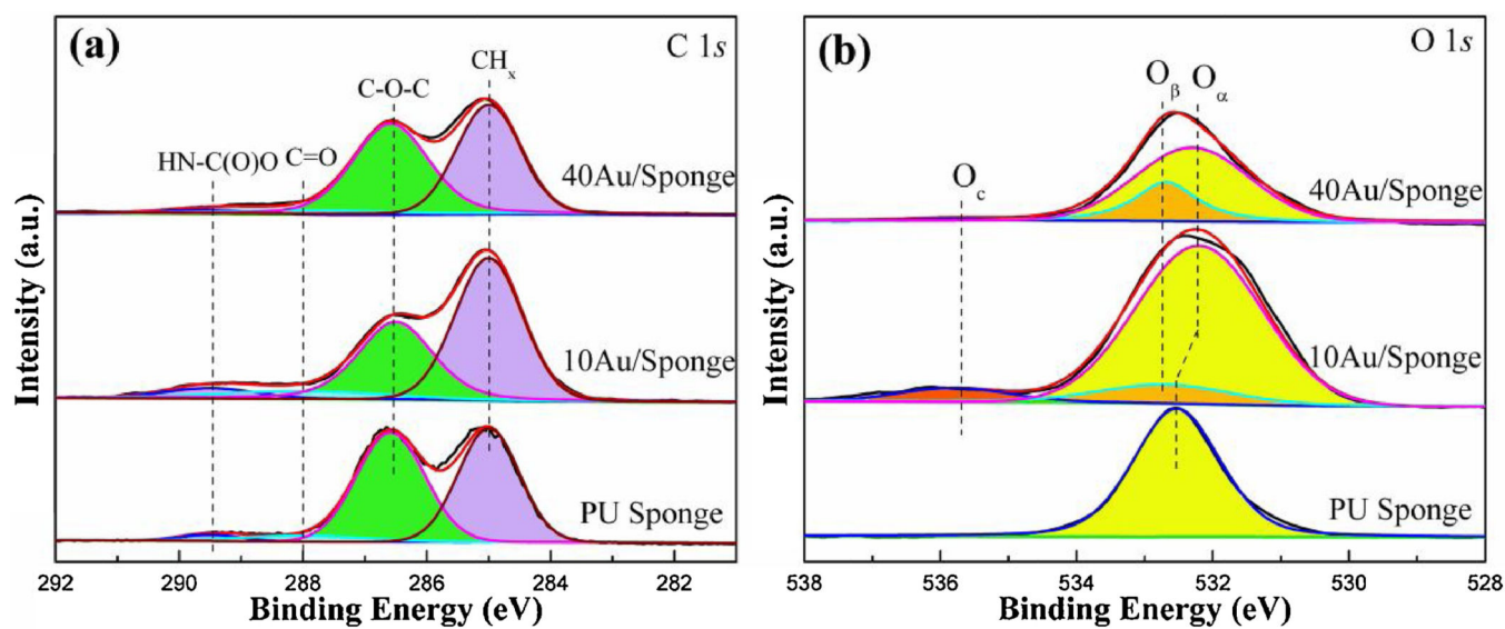
Fig.9. (a) C 1s and (b) O 1s XPS high-resolution scan spectra of PU sponge and AuNP/Sponge catalysts.
