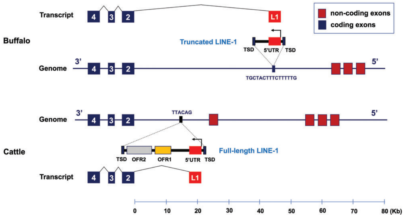
Fig. 6. Two independent LINE-1 insertions occurred in ASIP of water buffalo ( Bubalus bubalis ) and cattle ( Bos taurus ). The genomes, transcripts, and LINE-1 elements are represented 3′–5′ from left to right to be consistent with that in figure 2. The LINE-1 of cattle ASIP is based on Girardot et al. (2006).
