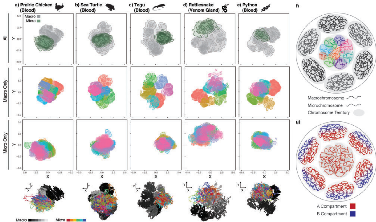
Fig. 3. Microchromosomes are likely co-localized in the 3D nucleus. (a–e) 3D interpretations of Hi-C interaction data shown as 2D point density plots from three distinct orientations for all chromosomes, macrochromosomes only, and microchromosomes only. For macro and micro only plots, different colors represent different chromosomes. Shown at the bottom are 3D interpretations of all chromosomes, with macrochromosomes in grayscale and microchromosomes in color. Additional orientations for each species are available in supplementary figures 4–8, Supplementary Material online. (f–g) Cartoon representations of a nucleus illustrating the hypotheses that (f) microchromosomes are centrally located in the nucleus and collectively inhabit a “microchromosome territory” and (g) that of spatial organization of A and B compartments in a nucleus containing A-rich microchromosomes.
