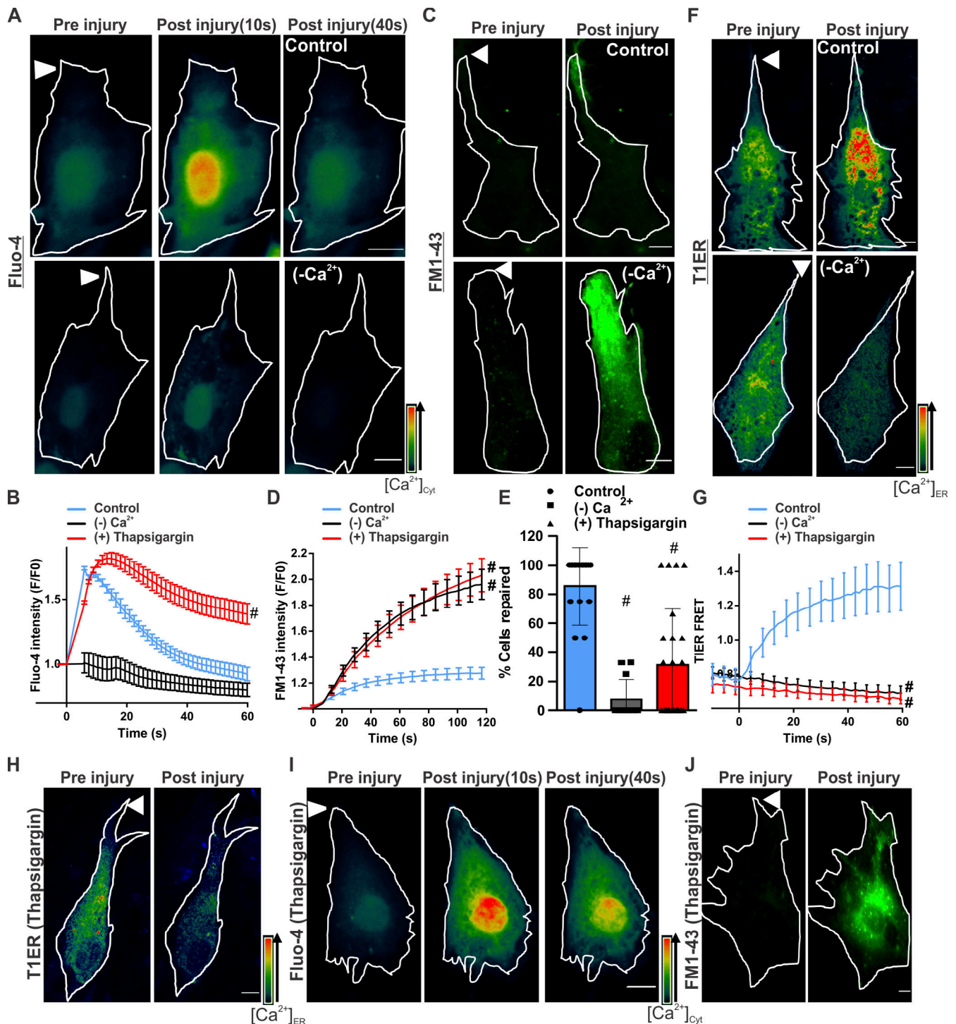
Figure 1. [Ca 2+ ] c homeostasis is required for PMR. (A) Healthy human myoblasts were labeled with Fluo-4 to monitor [Ca 2+ ] c following focal PM injury (arrowheads) by laser in the presence (control) or absence (-Ca 2+ ) of extracellular Ca 2+ . Pseudocolored images of the cell at different time points before and following injury are shown. Injury sites are marked with arrowheads. (B) Quantification of averaged kinetics for Fluo-4 intensity change in cells injured in the presence (control) or absence (-Ca 2+ ) of extracellular Ca 2+ or in the presence of SERCA inhibitor (1 mM TG). Plot shows mean ± SEM. n = 33 (control), 19 (-Ca 2+ ) and 29 (TG) cells; #, P < 0.0001. (C) Images showing FM1-43 dye entry into human myoblasts before and 60 s after focal laser injury in the presence (control) or absence (-Ca 2+ ) of extracellular Ca 2+ . (D) Quantification of FM1-43 dye entry kinetics in healthy myoblasts in the presence or absence of extracellular Ca 2+ or treated with 1mM TG in presence of Ca 2+ . Plot shows mean ± SEM. n = 16 (control), 25 (-Ca 2+ ) and 16 (TG) cells.; #, P < 0.0001. (E) Percentage of cells in C and D that successfully repaired. Plot shows mean ± SD. #, P < 0.0001. (F) Images before and 60 s after injury of human myoblasts expressing FRET-based ER calcium sensor T1ER, injured with (control) or without (-Ca 2+ ) extracellular Ca 2+ . (G) Quantification of normalized T1ER FRET ratios in cells injured as indicated. Plot shows mean ± SEM. n = 20 (control), 9 (-Ca 2+ ) and 17 cells (TG); #, P < 0.0001. (H-J) Images of human myoblasts labeled with T1ER (H), Fluo-4 (I), and FM1-43 (J) and treated with TG (1 mM) to inhibit SERCA. Images show the same cell before (preinjury) and 60 s (or indicated time points) after injury. Scale bars, 10 μm. Arrowhead indicates site of laser injury.
