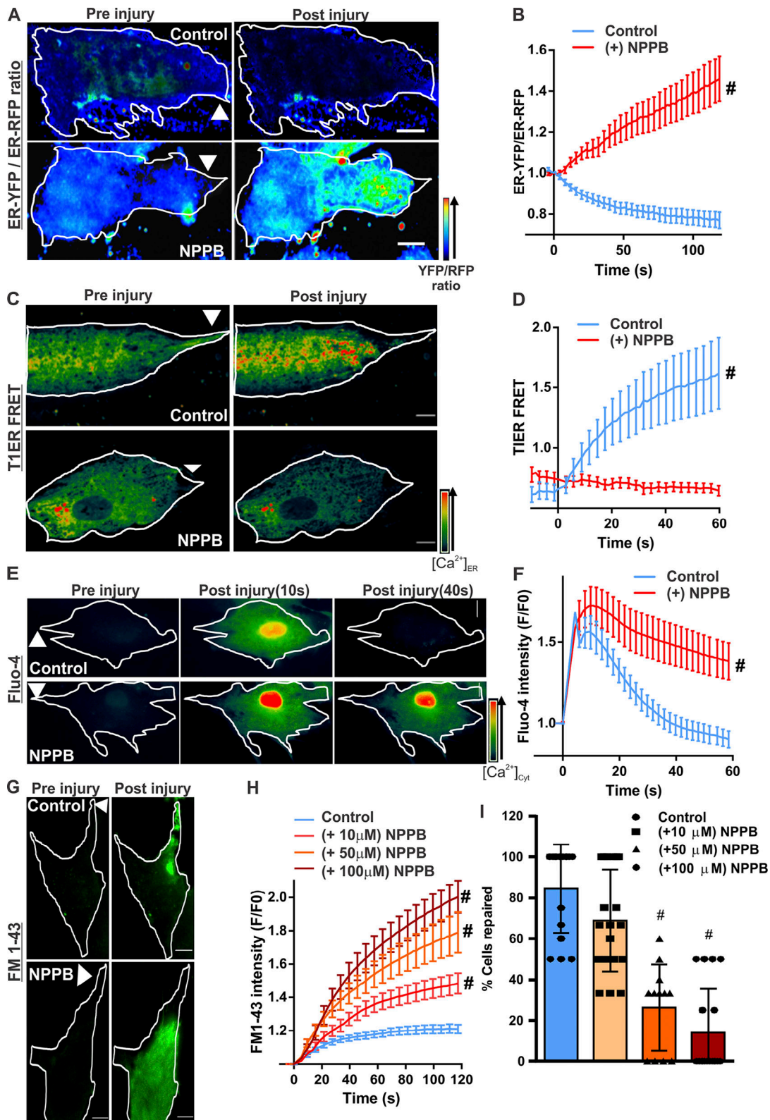
Figure 2. Ca 2+ homeostasis during PMR requires CaCC activity. Human myoblasts expressing KDEL-YFP and KDEL-RFP were treated with vehicle (control) or a CaCC blocker (50 μM NPPB). Quenching of YFP fluorescence by Cl - entry into the ER was monitored by ratiometric measurement of Cl - -sensitive YFP and Cl - -insensitive RFP fluorescence. (A) Pseudocolored images of cells before or 60s after laser injury (injury site marked by arrowheads). (B) Quantification of the normalized YFP/RFP ratio in control and NPPB-treated myoblasts. n = 18 (control) and 16 (NPPB) cells; #, P < 0.0001. (C and D) Pseudocolored images (C) and quantification (D) of T1ER FRET ratios before and after injury of myoblasts treated with vehicle (control) or NPPB (50 μM). Arrowheads indicate site of injury. n = 20 (control) and 17 (NPPB 50 μM) cells; #, P < 0.0001. (E and F) Pseudocolored images (E) and plots (F) showing change in [Ca 2+ ] c monitored by Fluo-4
