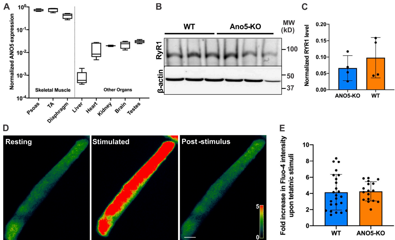
Figure S3. ANO5 expression and effect of its deficit on the ER Ca^{2+} -handling machinery. (A) Quantitative PCR analysis of ANO5 mRNA expression in various mouse tissues. (B and C) Western blot showing a representative blot (B) and quantification (C) of RYR1 levels in tibialis anterior muscles from WT and ANO5-KO mice. (D and E) Pseudocolored images (D) and plot (E) showing an increase in FDB myofiber Ca^{2+} levels in WT and ANO5-KO mice using Fluo-4 dye. Plots show mean \pm SD.
