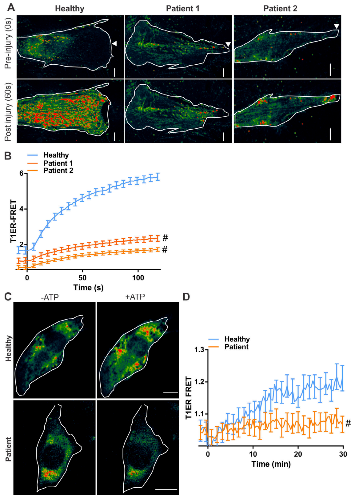
Figure S1. ANO5 deficit reduces ER calcium uptake following purinergic stimulation. (A and B) Healthy or ANO5-deficient patient fibroblasts expressing the ER calcium sensor T1ER were focally injured (arrowhead). Pseudocolored T1ER FRET images (A) and quantification (B) of normalized T1ER FRET, for cells before or following PM injury. n = 17 (healthy), 23 (patient 1), and 15 cells (patient 2). (C and D) Healthy or ANO5-deficient patient myoblasts expressing the ER calcium sensor T1ER were treated with ATP to induce \text{Ca}^{2+} entry into the cell. Pseudocolored T1ER FRET images (C) and quantification (D) of normalized T1ER FRET for cells before (-ATP) and 30 min following 50 \mu\text{M} ATP (+ATP) treatment. n = 21 (-ATP) and 17 cells (+ATP). Plots show mean \pm SEM. Scale bars, 10 \mu\text{m} . #, P < 0.0001 .
