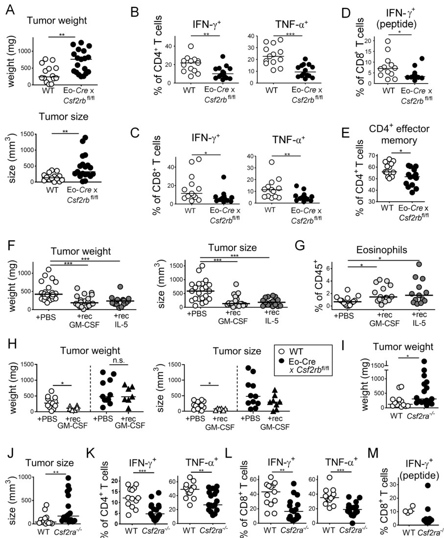
Figure 5. GM-CSF promotes tumor control through its activities on eosinophils. (A–E) Eo-Cre x Csf2rb fl/fl mice and their Cre-negative littermates were subcutaneously injected with 5 \times 10^5 MC38 cells and analyzed after 15 d with respect to their tumor weights and volumes (A) as well as their intratumoral frequencies of IFN- \gamma + and TNF- \alpha + CD4 + T cells (B), IFN- \gamma + and TNF- \alpha + CD8 + T cells (C; PMA/ionomycin), and IFN- \gamma + CD8 + T cells upon stimulation with MC38-specific peptide (D; n = 13 –14 tumors per genotype). Frequencies of effector memory cells are shown as well (E). Data in A–E are pooled from two independent studies. (F–H) WT C57BL/6 mice (F and G, n = 15 –22 tumors per group) and Eo-Cre x Csf2rb fl/fl mice and their Cre-negative littermates (H, n = 6 –14 tumors per group) were injected with MC38 cells and treated three times weekly with recombinant GM-CSF or IL-5 as indicated. The tumor weights and volumes at the study endpoint are plotted for two (IL-5) and three (GM-CSF) independently conducted, pooled studies in F and G and a representative study of two in H. (I–M) Csf2ra -/- mice and WT controls were injected with MC38 cells and analyzed after 15 d with respect to their tumor weights and volumes (I and J) and their intratumoral frequencies of IFN- \gamma + and TNF- \alpha + CD4 + T cells and of IFN- \gamma + and TNF- \alpha + CD8 + T cells (K and L; PMA/ionomycin, n = 13 –17), and of IFN- \gamma + CD8 + T cells upon stimulation with MC38-specific peptide (M; n = 4 –10). Data in I–L are pooled from three independent studies; data in M are from one representative study of three. *, P < 0.05 ; **, P < 0.01 ; and ***, P < 0.001 ; n.s., not significant; as calculated by Mann–Whitney test.
