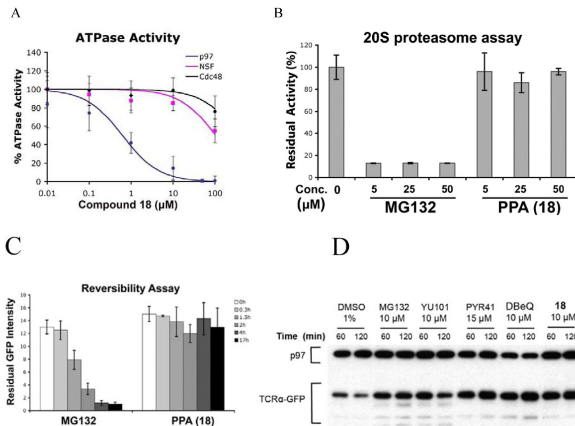
Figure 4. PPA inhibits p97 ATPase activity selectively and irreversibly. (A) Titration curves of the in vitro ATPase assays for PPA inhibition of p97, NSF, and Cdc48. (B) PPA did not inhibit human 26S proteasome activity. (C) Reversibility of PPA inhibition was determined using Ub G76V -GFP by washing out test compound and monitoring decay of GFP signal in the presence of cycloheximide for additional 17 h. (D) PPA block degradation of an ERAD substrate, TCR \alpha -GFP stably expressed in HEK293 cells. Cells were incubated with MG132, washed and treated with cycloheximide plus compound for 60 min or 120 min. Samples were immunoblotted with anti-p97 as loading control and anti-GFP antibody to detect TCR \alpha -GFP.
