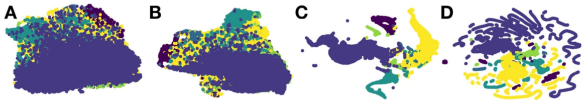
Fig. 3. UMAP projection of penultimate layer of neural network for one select colon slide; nodes colored by true sub-compartment; a) ImageNet-pretrained CNN embeddings of patches; b) colon-pretrained CNN embeddings of patches; c) updated GNN patch embeddings after ImageNet extraction; d) updated GNN patch embeddings after colon-pretrained CNN extraction
