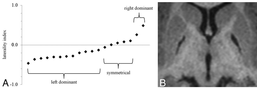
FIG 2. Laterality of GP infarcts. A, Most GP infarcts were left-dominant. A few were nearly symmetrical (5 were within \pm 10\% ), and 2 were right-dominant. The average laterality index was -0.13 , and the median was -0.17 . B, An example of a left-dominant infarct. The laterality index in this case is -0.20 .
