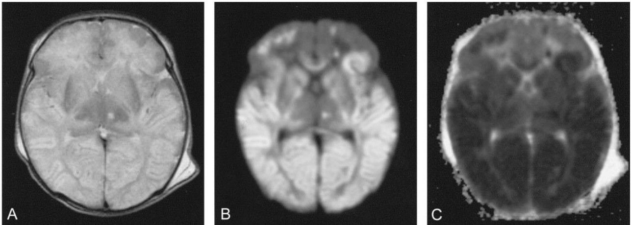
FIG 1. Images from the case of a 8-day-old girl with citrullinemia. MR imaging was performed 2 days after a blood ammonia peak of 2083 \mu\text{mol/L} .
