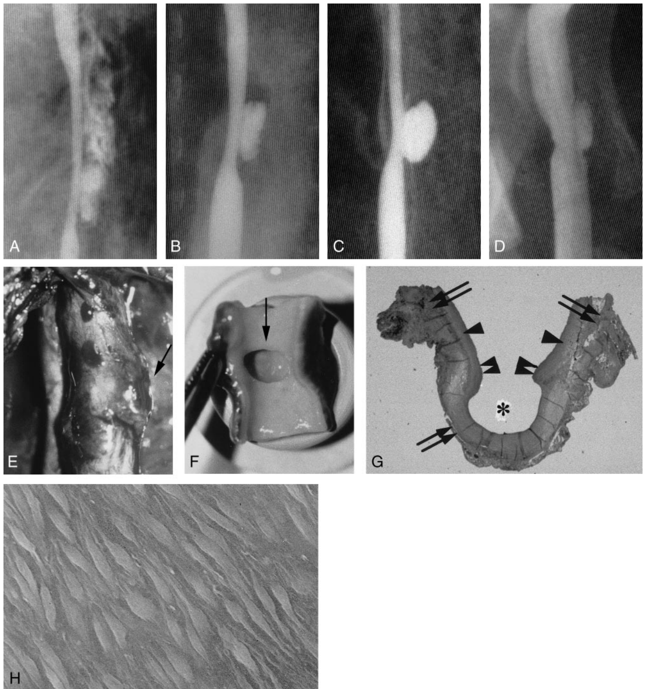
FIG 3. Example of aneurysm formation, with persistent stenosis (group I-C 6-mm elliptical defect). A, Angiogram shows a double shadow due to a massive adventitial hematoma that formed immediately after lesion creation. B, Angiogram obtained 2 hours later shows a subadventitial hematoma with the characteristics of an aneurysmal pouch. C, Angiogram obtained 1 week later shows that the hematoma has become a saccular aneurysm. D, Chronic-stage (3-month) angiogram shows that the aneurysm is smaller. E, Photograph shows external protrusion of the aneurysm (arrow). F, Chronic-stage photograph obtained in shows that part of the intimal defect extends to the aneurysm orifice (arrow). G, Chronic-stage photomicrograph shows that the inner layer of the aneurysm dome (asterisk) is covered with organized clots and fully endothelialized (elastica van Gieson stain, original magnification \times 5 ). Arrows indicate the adventitia; single arrowheads, media; double arrowheads, intima. H, Scanning electron micrograph shows endothelialization (original magnification \times 700 ).
