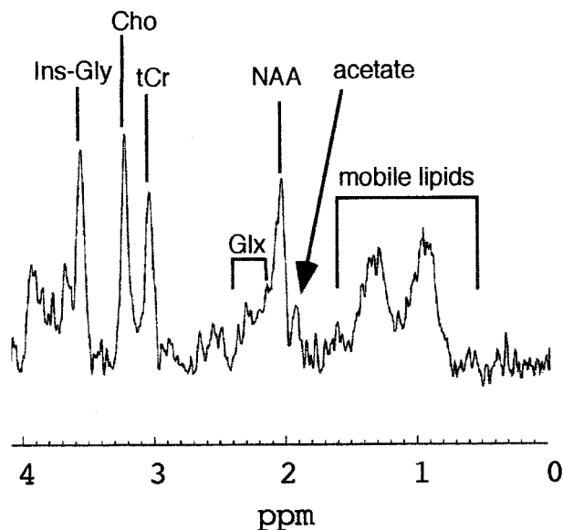
FIG 2. ^1\text{H} MR spectrum obtained at with the STEAM sequence (TE, 20 milliseconds) in the occipitoparietal white matter. The dominant feature of the spectrum is the high lipid and Ins-Gly content. The presence of an unusual resonance at 1.95 ppm was detected and assigned to acetate.
