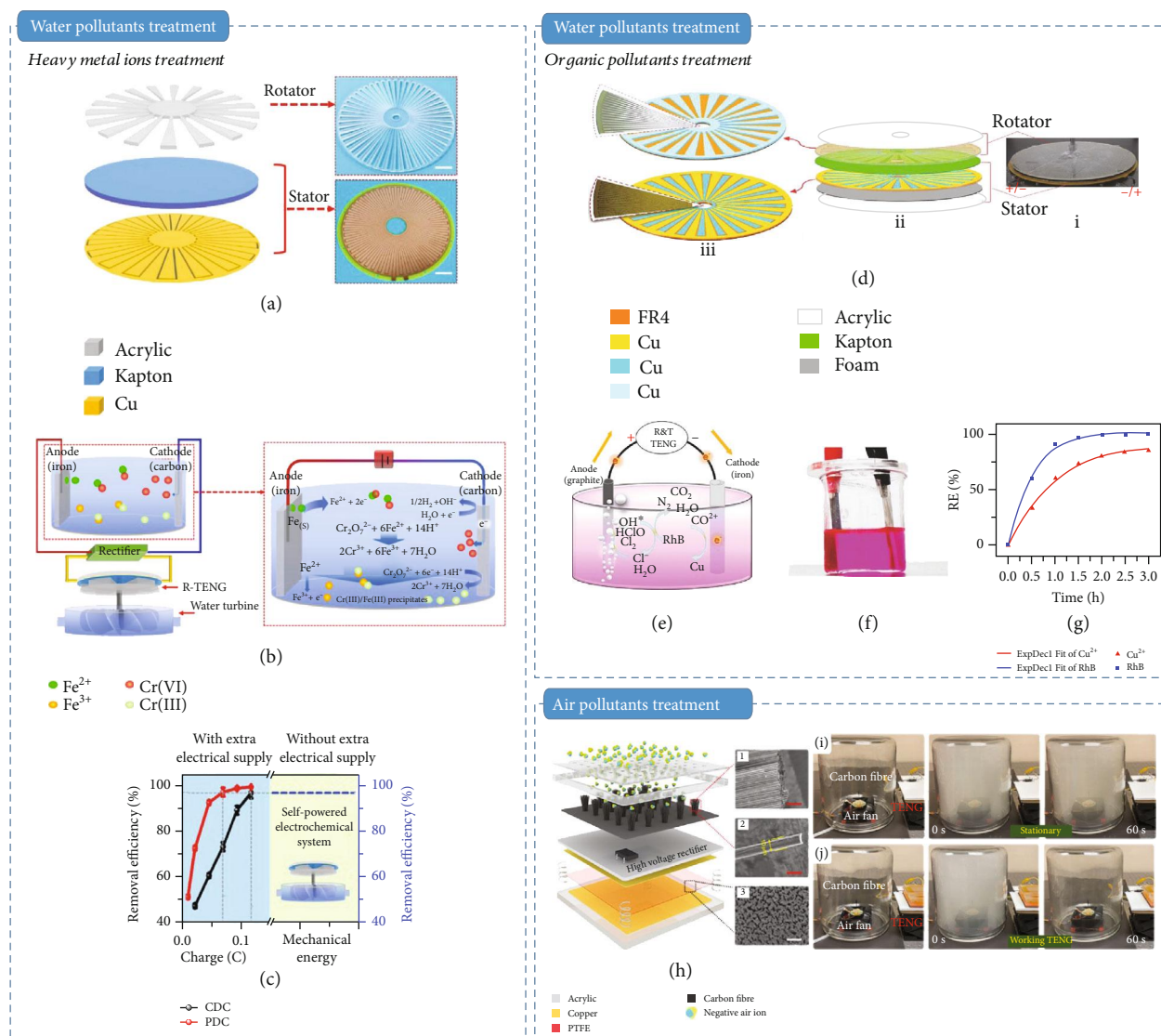
FIGURE 2: Self-powered electrochemical pollutant treatment: (a) sketch map of rotary TENG; insert displays the pictures of stator and rotator; (b) SP system for removing Cr(VI) powered by rectified TENG; (c) the comparison of charge consumption for Cr(VI) removal under different conditions [50]; (d) sketch map of the rotary TENG; (e, f) the mechanism image and optical image of SP electrochemical system for cupric ions and rhodamine B removal; (g) removal efficiency of cupric ions and rhodamine B [54]; (h) sketch map of the triboelectric negative air ion generator; (i, j) the contrast photographs of the smog cleaning by the MSNG in stationary conditions (i) and with the FS-TENG conducting at 0.25 Hz (j) [63].
