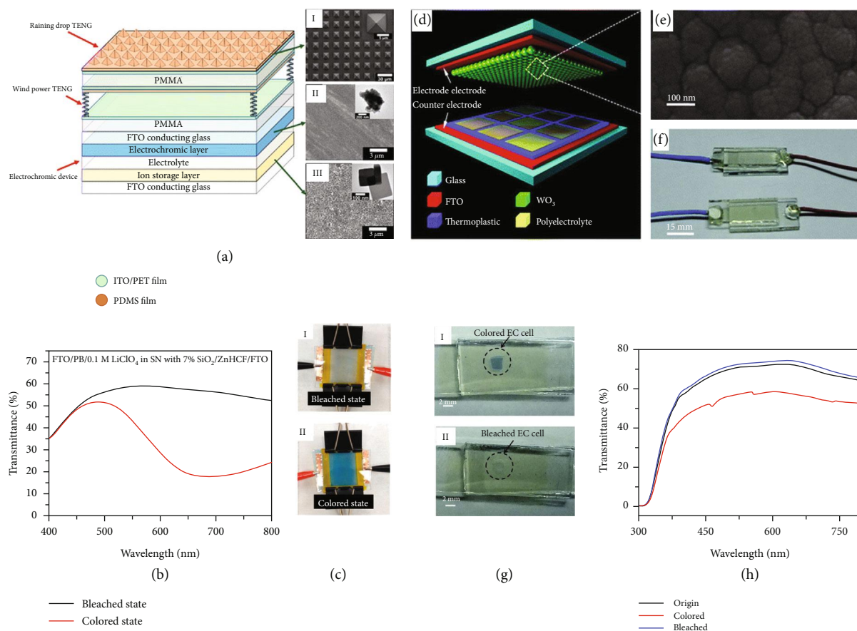
FIGURE 5: Self-powered electrochromic reaction: (a) schematic diagram of the SP smart window integrated with a raindrop-TENG, a wind-powered-TENG, and an electrochromic device from the top to the bottom; inserts are the SEM images of (I) PDMS film, (II) PB film, and the (III) ZnHCF film; (b) transmittance spectra and (c) photographs of the SP smart window system in bleached and colored states [99]; (d) the schematic structure of the WO_3 -based SP electrochromic device; (e) SEM image of the WO_3 film; (f) the photographs of the EC WO_3 -based SP electrochromic device; (g) color changing images of the WO_3 -based SP electrochromic device; (h) transmittance spectra of the WO_3 -based SP electrochromic device [100].
