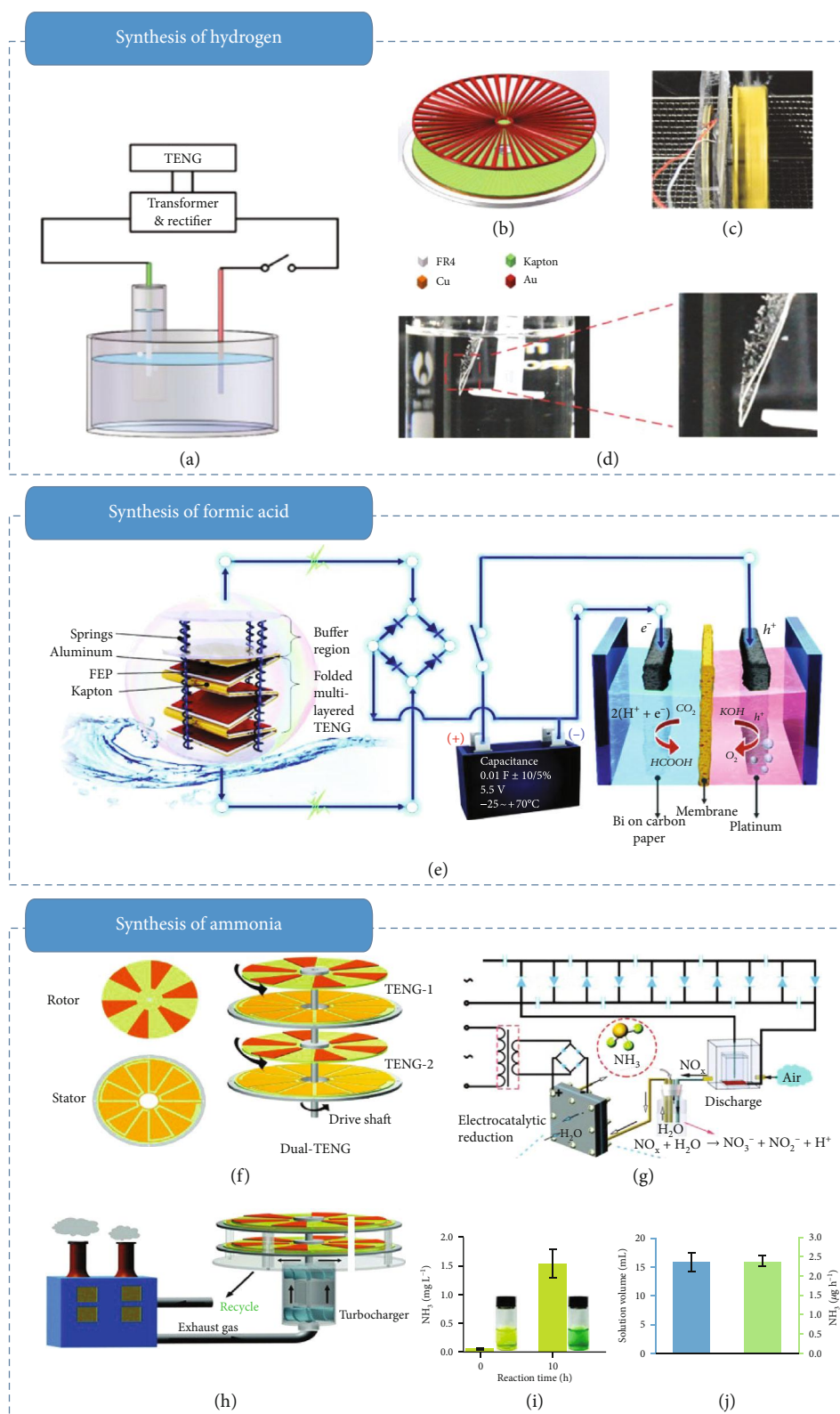
FIGURE 3: Self-powered electrochemical synthesis: (a) sketch map of the SP water splitting system; (b) structure of the disk TENG; (c) the SP water splitting system driven by a miniature water turbine; (d) images of the system with bubble producing [74]; (e) sketch map of the SP electrochemical system for \text{CO}_2 reduction powered by TENG for harvesting ocean-wave energy [70]; (f) sketch map of the designed TENG; (g) reaction of SP ammonia synthesis powered by TENG; (h) sketch map of the SP structure driven by exhaust gas; (i, j) concentration of \text{NH}_3 in the cathode compartment at different times (i) and the volume of residual solution and the yield of \text{NH}_3 (j) by the SP system after ten hours [82].
