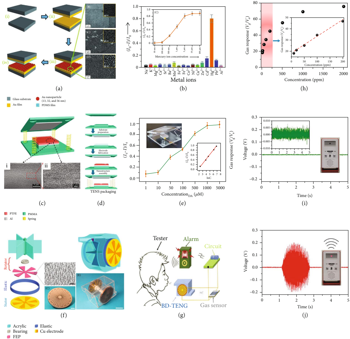
FIGURE 4: Self-powered electrochemical sensor: (a) fabrication process and the structure of the TENG; (b) selectivity of the SP electrochemical sensor for testing Hg^{2+} ions. Inset shows the sensitivity of Hg^{2+} ions detection [93]. (c, d) Sketch map and the fabrication process of the TENG; (e) sensitivity of the SP active sensor in supervising dopamine. Insets show the structure of designed TENG and proportional relation between output performance of TENG and the concentration of dopamine [94]. (f) Sketch map of the blow-driven TENG; (g) a schematic illustration the blow-driven TENG using as an SP breath analyzer; (h) response curve of the measured gas in terms of output voltage. Inset is the schematic illustration of a self-power breath analyzer; (i, j) voltage signals of the system with warning alarm by a person before and after drinking alcohol [95].
