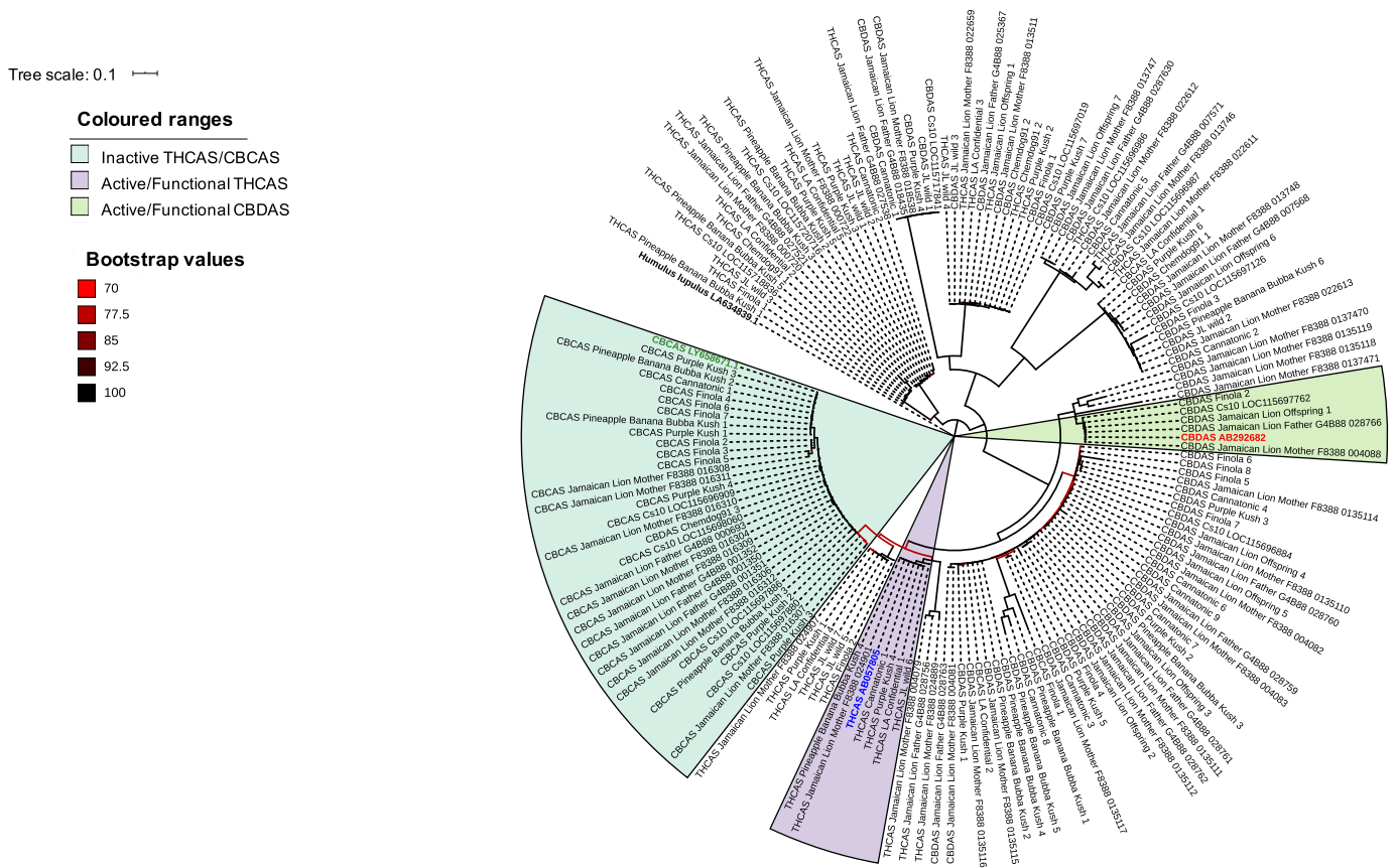
Fig. 4 Maximum-likelihood phylogenetic tree depicting the relationship among the Cannabis sativa cannabinoid synthase genes tetrahydrocannabinolic acid synthase ( THCAS ), cannabidiolic acid synthase ( CBDAS ) and cannabichromenic acid synthase ( CBCAS ). The published nucleotide sequences of the active/functional forms of THCAS (GenBank acc. no. AB057805.1), CBDAS (GenBank acc. no. AB292682.1), CBCAS (GenBank acc. no. LY658671.1) and the paralogues of these genes as annotated in the cs10 v.2.0 and Jamaican Lion (female parent and male parent) assemblies (Supporting Information Tables S1, S2) were aligned against the latest C. sativa reference genome assemblies (Table 1) using BLAST+/2.2.29 (Altschul et al. , 1990). Best hits corresponding to a percentage identity > 98.5%, query coverage > 75% and alignment length = query length \pm 100 bp were retained (Tables S1, S2). The nucleotide sequences of these best hits were extracted from each assembly (where applicable) using BEDTools v.2.26.0 (Quinlan & Hall, 2010). TRANSDCODER v.3.0 was used to predict the longest open reading frame from the extracted regions ( https://transdecoder.github.io/ ). The predicted proteins along with amino acid sequences (complete CDS) of AB057805.1 (gene ID in blue), AB292682.1 (gene ID in red), LY658671.1 (gene ID in green) and the other cannabinoid synthase gene copies annotated in the cs10 v.2.0 and Jamaican Lion (female parent and male parent) genome assemblies were used for multiple sequence alignment using CLUSTAL Omega (Sievers et al. , 2011). The phylogenetic tree was reconstructed from these alignments using RAxML v.8.12.12, with 500 bootstrap replicates under the JTT model of amino acid substitution and visualized using Interactive Tree Of Life (iTOL) (Letunic & Bork, 2007; Stamatakis et al. , 2008). The tree was rooted with the Humulus lupulus THCAS homolog (GenBank acc. no. LA634839.1). Only bootstrap values of > 70% are shown. It is worth noting that all CBCAS genes cluster with some the THCAS genes reflecting the high sequence similarity between these two cannabinoid synthase genes (Fig. 3).
