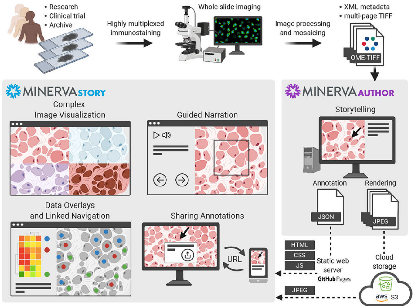
Figure 1: Minerva Workflow.
