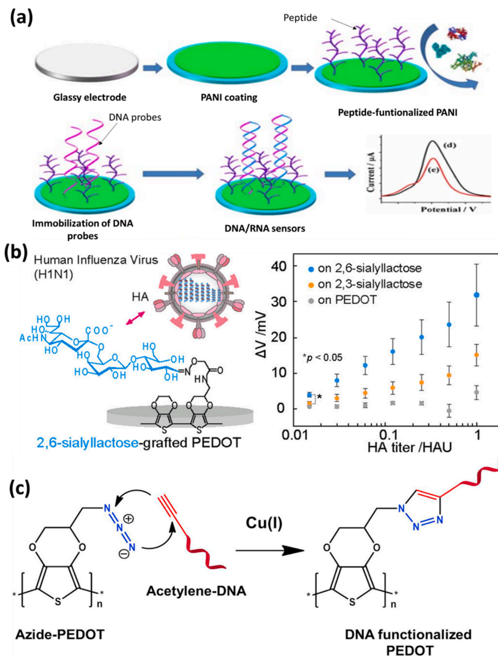
Fig. 4. (a) Schematic illustration of the preparation process of antifouling RNA biosensors using peptides for surface modification of PANI polymer. Reproduced with permission from (Wang et al., 2020a); (b) Biosensor based on PEDOT grafted sialyllactose for human influenza A virus detection. Reproduced with permission from (Hai et al., 2017); (c) Functionalization of PEDOT for DNA biosensor using CuAAC reaction. Reproduced with permission from (Galán et al., 2015).
