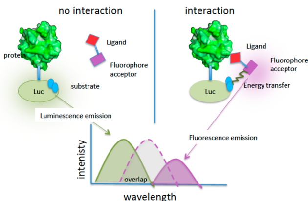
Figure 14. Description of BRET experiments for target engagement with no interaction (left) and interaction (right): Luc, luciferase; green line = donor emission spectrum; violet dot line = acceptor excitation spectrum; violet line = acceptor emission spectrum.
