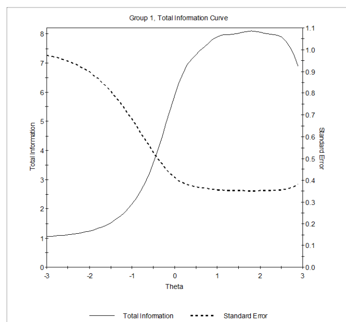
Figure 1. Test information function (TIF) of the BFAS under the graded response model (GRM). Latent trait ( \theta ) is shown on the horizontal axis, and the amount of information and the standard error yielded by the test at any trait level are shown on the vertical axis.
