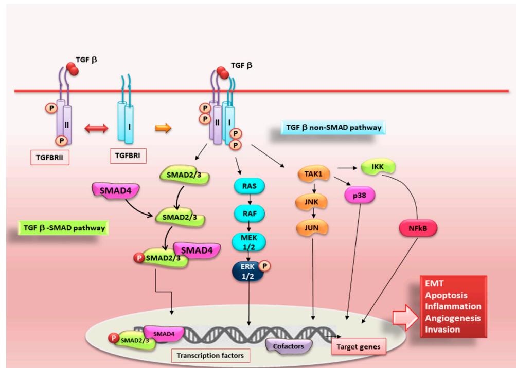
Figure 2. Schematic illustration of canonical and non-canonical TGF- \beta signalling pathways. Canonical SMAD-dependent TGF- \beta signalling is initiated by TGF- \beta ligand binding to receptors TGFBR1/R2, which once activated, lead to the phosphorylation and activation of SMAD2/3 which, in turn, binds to cofactor SMAD4. The trimeric SMAD complex translocate into the nucleus, where they interact with other transcription factors to regulate target gene expression. In the SMAD-independent pathways, the TGF- \beta receptor complex transmits its signal through other factors, such as RAS-RAF-MEK-ERK. Once activated, ERK1 and ERK2 can facilitate EMT by increasing the expression of EMT transcription factors. Moreover, activated TAK1/JNK/JUN factors act to regulate cellular apoptosis and proliferation, whereas they can also mediate metastasis, angiogenesis and cellular growth through other transcription factors.
