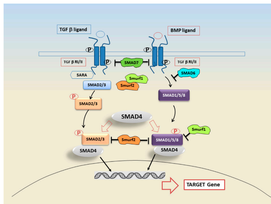
Figure 1. TGF- \beta signalling is triggered through BMP or TGF- \beta ligands. Ligands bind the TGF- \beta receptor II (TGF- \beta R-II) which recruits and phosphorylates TGF- \beta receptor I (TGF- \beta R-I). In the TGF- \beta signalling pathway, TGF- \beta R-I phosphorylates the SMAD2 and 3, or SMAD1, 5, and 8. The cofactor SMAD4 forms a heterotrimeric complex with SMAD2/3 and SMAD1/5/8. Activated SMAD complex, translocate into the nucleus interacting with transcription factors and modulating or repressing the gene transcription. Feedback regulation is mediated by inhibitory SMAD 6/7. Both SMAD6 and SMAD7 are in turn induced by TGF- \beta receptors and regulated through the help of SMAD ubiquitination regulatory factors (Smurfs) 1 and 2.
