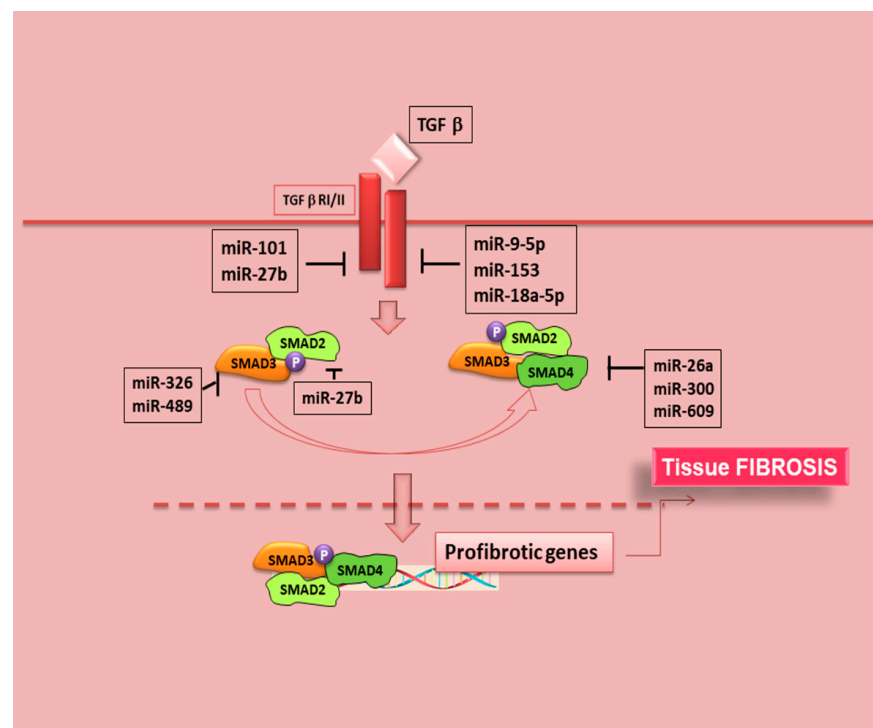
Figure 4. Modulation of the TGF- \beta signalling pathway by miRNAs. In response to TGF- \beta signal, the expression of a cohort of miRNAs is modulated. Several miRNAs are involved in the process of EMT-dependent tissue fibrosis by targeting components of the TGF- \beta signalling pathway.
