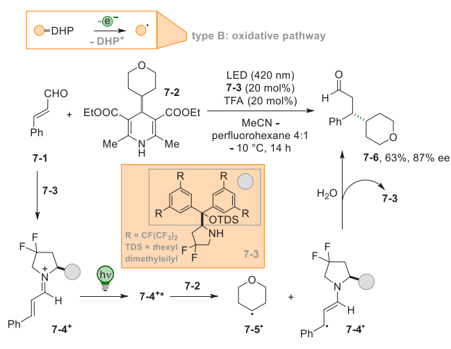
Scheme 7. Alkyl-DHPs as Radical Precursors in Combination with Iminium Catalysis
