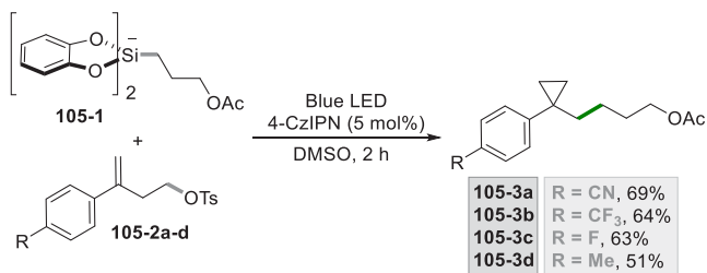
Scheme 105. Synthesis of 1,1-Disubstituted Cyclopropanes
