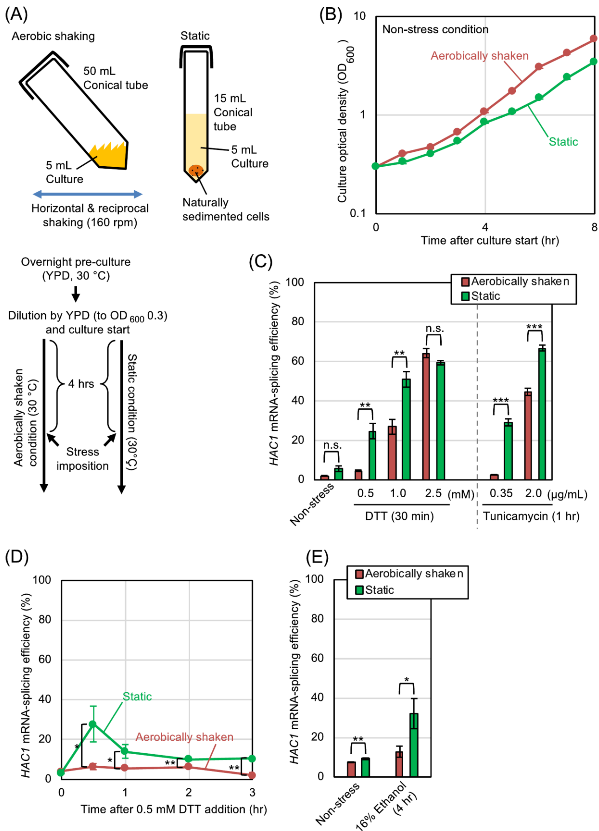
FIGURE 1: HAC1 -mRNA splicing is compromised by aerobic agitation. (A) Procedures for culturing and ER-stress induction of S. cerevisiae cells under the aerobically shaken condition or under the static condition. ER-stress agents (DTT, tunicamycin, or ethanol) were added to the media 4-hr after culture start. (B) Optical density of cultures (wild-type BY4742 cells) was monitored under non-stressing conditions. (C-E) Wild-type BY4742 cells were cultured and were ER-stressed (or remained non-stressed) as shown in panel A, and were checked for HAC1 -mRNA splicing. n.s. (not significant): p > 0.05 , *: p < 0.05 , **: p < 0.01 , ***: p < 0.001 .
