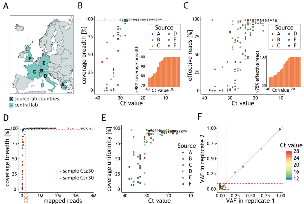
Fig. 4. Viral genotype assignment in clinical samples reflects global genome diversity. (A) The multicentre study involved six laboratories, located in different European countries, which generated datasets analysed at a central location (SOPHiA GENETICS, Switzerland). (B) Fraction of viral genome covered by at least ten reads (y-axis) as a function of the cycle threshold (Ct) value (x-axis). Each point represents the results for a sample, colour-coded according to the source lab. The dashed line indicates 98% coverage breadth. The percentage of samples with at least 98% genome coverage breadth (y-axis) below a given Ct (x-axis) is represented in the inset. (C) Fraction of effective reads mapping to the genome of severe acute respiratory syndrome coronavirus 2 (SARS-CoV-2) (y-axis) as a function of the Ct value of the clinical samples (x-axis). Each point represents the results for a sample colour-coded according to the source lab. The percentage of samples with at least 75% effective reads (y-axis) below a given Ct (x-axis) is represented in the inset. (D) Fraction of viral genome covered by at least ten reads (y-axis) as a function of the number of reads mapping to the SARS-CoV-2 genome (x-axis). Each point represents a sample and is colour-coded according to its Ct value. The horizontal dotted line indicates 98% coverage breadth and vertical dotted line indicates 200K mapped reads. (E) Percentage of genome coverage uniformity (y-axis) as a function of the sample Ct value (x-axis). Each point represents the results for a sample colour-coded according to the source lab. (F) Relationship between variant fraction for variant calls in clinical samples processed in replicates and with genome coverage breadth >98%. Dotted lines demarcate variant allele fraction (VAF) = 0.1. Variants are coloured based on the Ct value of the replicate.
