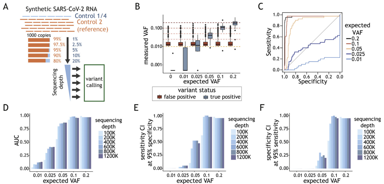
Fig. 3. Determination of assay parameters for reliable intra-host variability detection. (A) Schematic representation of the experimental design. Varying amounts of SARS-CoV-2 (severe acute respiratory syndrome coronavirus 2) Control 1 or 4 (blue) were mixed with SARS-CoV-2 synthetic genome reference (Control 2) to obtain desired variant allele fractions (VAFs) (0.01–0.2). One thousand viral genome copy mixes (g.c.p.r.) were spiked into human RNA. Variant calling was performed at varying sequencing depths. (B) Distribution of variant fraction measured for known (true positives, blue) and background (false positives, red) variants (y-axis) as a function of the expected VAFs in the samples (x-axis). The black horizontal line in the boxplot indicates the median and the whiskers the 5% and 95% quantiles. (C) Sensitivity (y-axis) as a function of the specificity (x-axis) with VAF value used as a predictor for true variant calls. The ROC curves are colour-coded depending on the expected VAF of the known variants in each experiment. (D) Area under the ROC curve (AUC) (y-axis) as a function of the expected VAF of the variants (x-axis) at sequencing depth between 100K and 1200K reads. Colour code for analysis done with samples at different sequencing depth is depicted on the right. (E) Sensitivity CI (confidence interval) calculated at 95% specificity (y-axis) and (F) specificity CI at 95% sensitivity (y-axis) as a function the expected VAF for the variant (x-axis). Colour code for analysis done at different sequencing depths is depicted on the right.
