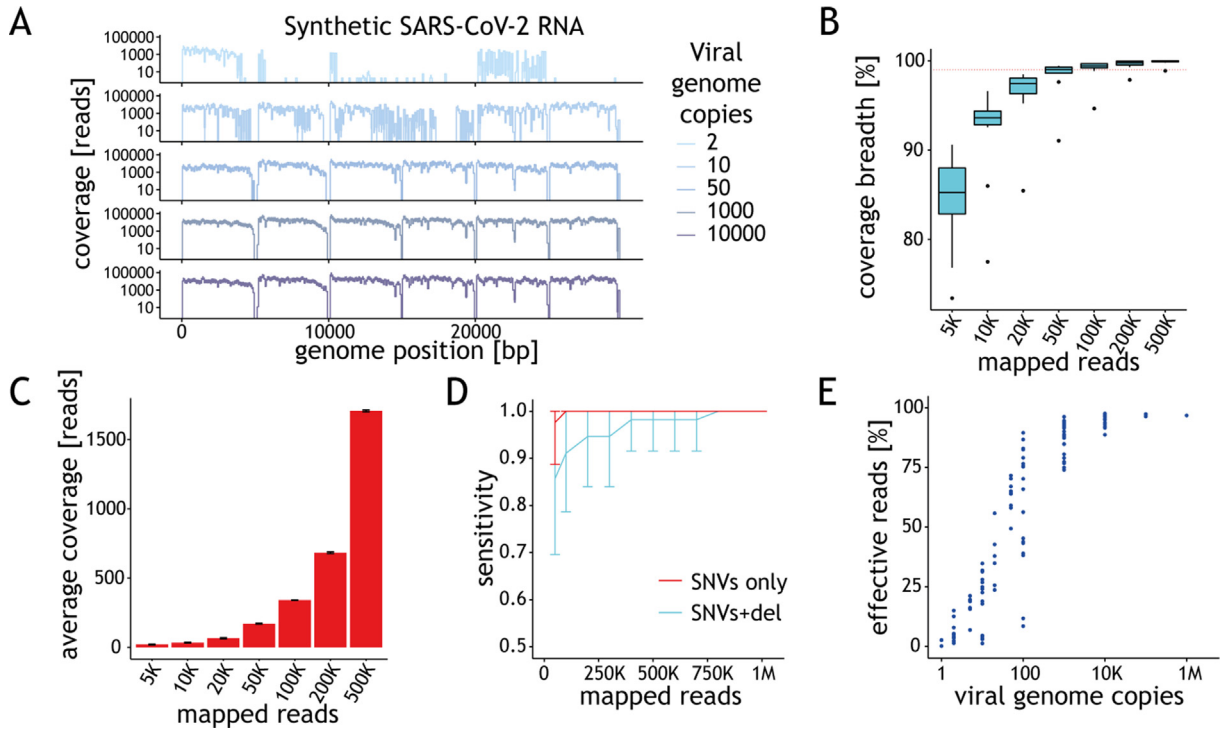
Fig. 2. Performance of the assay depends on the amount of starting material. (A) Ideograms depicting the genome coverage (y-axis) for representative samples with varying amount of synthetic viral genomes (x-axis). Signal drops every 5 kb are expected due to gaps in the reference material. (B) Distribution of the genome coverage breadth (y-axis) as a function of the number of mapped reads for samples with 10 000 genome copies per reaction (g.c.p.r.). Horizontal dashed line depicts 98% coverage breadth. The horizontal line in the boxplot indicates the median and the whiskers the 5% and 95% quantiles. (C) Average coverage depth across synthetic severe acute respiratory syndrome coronavirus 2 (SARS-CoV-2) genome (y-axis) as a function of the number of mapped reads (x-axis) based on data from samples with 10 000 g.c.p.r. (D) Average sensitivity of variant calling for single nucleotide variants (SNVs) (red) or SNVs + 10 bp indel (cyan) in SARS-CoV-2-c1 (y-axis) as a function of the number of mapped reads based on the results obtained for samples with at least 98% genome coverage breadth. Error bars represent standard deviation. (E) Percentage of effective reads (y-axis) shown as a function of the viral load (g.c.p.r.) in the sample. Each point represents the data for one sample.
