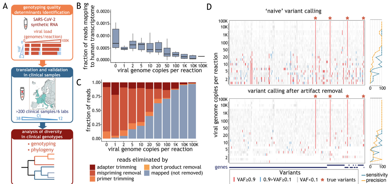
Fig. 1. Artefact removal is a prerequisite for reliable variant calling. (A) Schematic representation of the study. In experiments using synthetic severe acute respiratory syndrome coronavirus 2 (SARS-CoV-2) RNA, we varied a number of experimental parameters—including viral load, variant allele fraction (VAF) and sequencing depth—and determined which of these factors critically impact(s) genotyping quality (top box). We validated these metrics using data obtained from clinical samples, whose viral load is reflected by the cycle threshold (Ct) value (middle box). We determined the phylogeny of all clinical samples that met our guidelines (bottom box). (B) Distribution of the fraction of raw reads aligning to human transcriptome (y-axis), obtained with STAR aligner, as a function of the number of synthetic viral genome in the sample (x-axis). The horizontal line in the boxplot indicates the median and the whiskers the 5% and 95% quantile. (C) Average fraction (from at least three replicates) of sequencing reads that mapped to the SARS-CoV-2 genome or were the result of different technical artefacts (y-axis) for samples with varying amounts of synthetic viral genomes (x-axis). (D) Ideogram depicting the location of variants detected in samples with a varying number of synthetic viral genomes (denoted on the left) before (top panel) and after (bottom panel) removal of reads labelled as technical artefacts. Variants with allele fraction <0.1, between 0.1 and 0.9, and >0.9 are shown in grey, blue and red, respectively. Expected SARS-CoV-2 variants present in the control are marked with asterisks. Plots on the right show sensitivity and precision of the variant calls.
