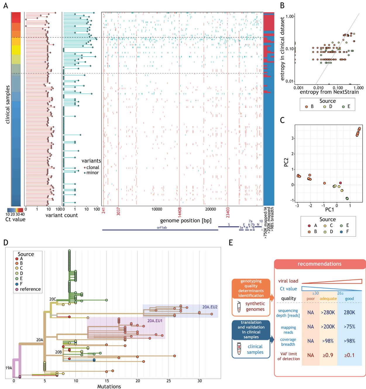
Fig. 5. Variant frequencies found in the clinical dataset reflect global frequencies. (A) Summary of the variant calling analysis for all unique clinical samples (rows) sorted by the cycle threshold (Ct) value (left). The horizontal dashed lines indicate Ct values of 26 and 30. The numbers of clonal (variant allele fractions, VAF \geq 0.9 , red) and minor ( 0.1 < \text{VAF} < 0.9 , cyan) variants for each sample are represented as horizontal bar-plots (middle left). The position of each clonal (red) and minor (cyan) variant is displayed along the genome (middle right). Coordinates marked in red indicate positions of the most prevalent variants. Classification of the samples relative to the different recommendations (listed below each column) (right): blue indicates the recommendation was fulfilled and red that it was not. (B) Relationship between the entropy estimated for all clonal variants in clinical samples (y-axis) and the entropy of the same variants in samples collected in the same country and during the same period according to Nextstrain [30] (x-axis). Only samples with >200 K effective reads and 98% coverage breadth from centres with data for more than 15 samples were considered in this analysis. (C) 2-D principal component analysis results of clonal variants in clinical isolates (points). Points are coloured based on the sample source. (D) Phylogenetic tree of all clinical isolates with >200 K effective reads and 98% coverage breadth criteria. Samples are coloured according to the source. Clades (according to Nextstrain) are indicated. Samples corresponding to subclade 20A.EU.1 and 20A.EU.2 are highlighted by red and blue boxes, respectively. Length of the branches reflects the number of mutations (x-axis). The tree visualization was generated using the Nextstrain platform [30]. (E) Schematic representation of the recommendations for reliable genotyping with amplicon-based approach. We used synthetic viral genomes to determine the minimal viral load and VAF. We validated these recommendations and made them broadly applicable using clinical samples by determining the minimal sequencing depth, fraction of mapped reads and coverage breadth. Samples were classified into three quality categories based on their viral load: good ( \geq 1000 genome copies per reaction (g.c.p.r.), adequate (uncertain g.c.p.r., Ct values in the range 26–30) and poor ( <100 g.c.p.r., typically value Ct > 30 ).
