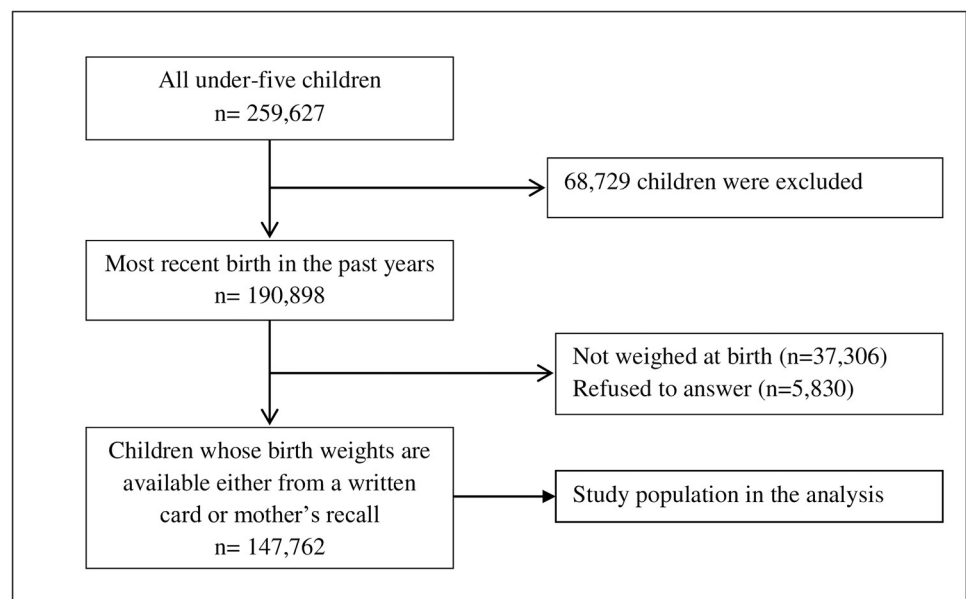
Fig 2. Selection of study participants, NFHS-4.
