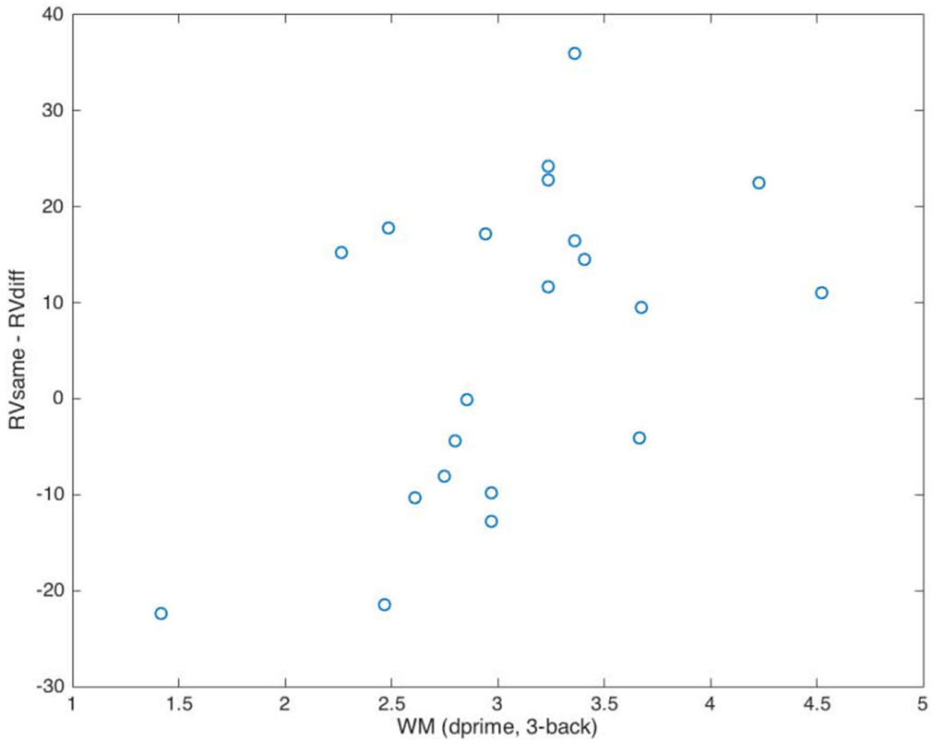
Figure 2. Correlation between source analysis model fit and WM. For the N1 time window, correlation between WM as measured by d' on a 3-back task, and the difference in the goodness of fit of a parietal source model to scalp topography data between same and different talkers ( RV_{same} - RV_{diff} ).
