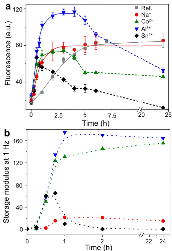
Figure 7. (a) Effect of metal ions (Na + , Co 2+ , Al 3+ , and Sn 4+ at 120 mM) on the kinetics of WPI fibril formation at pH 2, 90 °C, measured by ThT fluorescence at 485 nm. (b) Gelation data for WPI solutions with metal ions at 120 mM.
