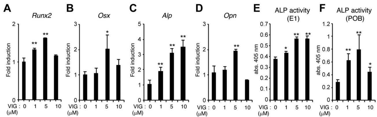
Figure 2. Vignacyanidin (VIG) stimulates osteoblast differentiation of osteoblast-lineage cells. (A-E) MC3T3-E1 cells were cultured in osteogenic medium (growth medium supplemented with 50 μg/ml ascorbic acid, and 10 mM β-glycerophosphate) with 0, 1, 5, or 10 μM VIG for 7 days. The mRNA levels of Runt-related transcription factor 2 ( Runx2 ) (A), Osterix ( Osx ) (B), Alkaline phosphatase ( Alp ) (C), and Osteopontin ( Opn ) (D) were determined by quantitative real-time polymerase chain reaction. ALP activity was also assessed (E). Primary cultured calvarial osteoblasts were treated with 0, 1, 5, or 10 μM VIG along with 10 mM β-glycerophosphate and 50 μg/ml ascorbic acid for 7 days, and ALP activity was assessed (F). Data are presented as mean±SD (n=4). **p<0.01, *p<0.05, versus control treatment.
