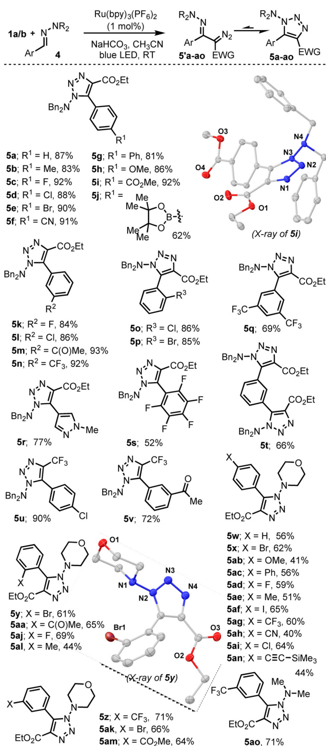
Scheme 2. Synthesis of 1,2,3-triazoles 5a–ao and molecular structure of compounds 5i and 5y in the solid state. Anisotropic displacements shown at 50% probability level. [16]
