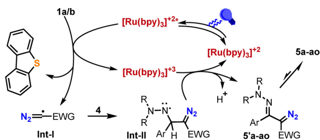
Scheme 3. Plausible reaction mechanism for the formation of 5a–ao .
