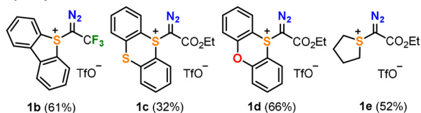
Scheme 1. Synthesis of \alpha -diazo sulfonium triflates 1a–e .
