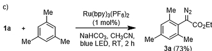
Figure 3. a) DSC analysis for 1a in air; b) Quenching of the fluorescence of [Ru(bipy) 3 ][PF 6 ] 2 following the addition of 1a ; c) trapping the postulated diazomethyl radical intermediate with 1,3,5-trimethylbenzene to afford product 3a and formation of diethyl acetylenedicarboxylate via radical dimerization and dinitrogen elimination.
