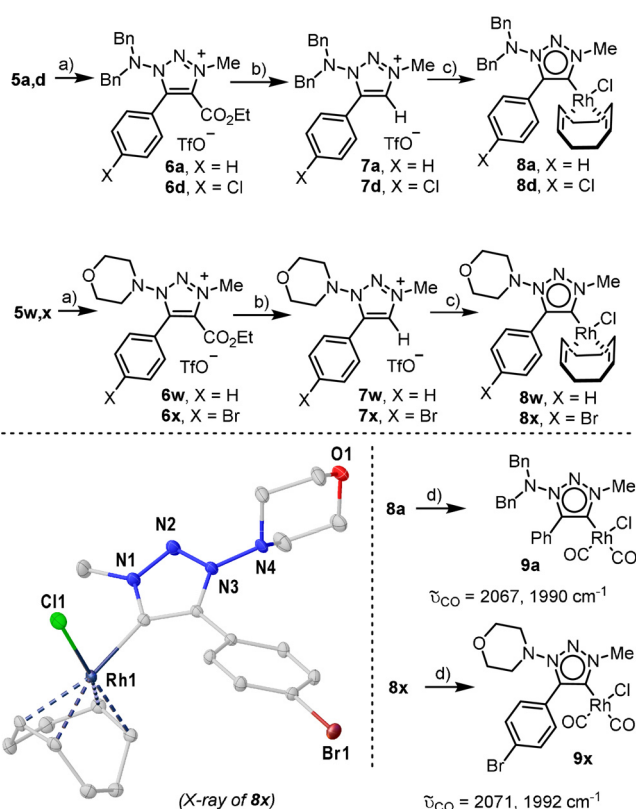
Scheme 4. Synthesis of Rh complexes 8a,d,w,x via decarboxylative metalation, evaluation of the donor properties of the new ligands and molecular structure of 8x . Anisotropic displacements shown at 50% probability level and H atoms removed for clarity. [16] Reaction conditions: a) MeOTf (1.2 equiv), DCM, 8 h, 0^\circ\text{C} \rightarrow \text{r.t.} ; b) (LiOH 3.0 equiv), THF/ \text{H}_2\text{O} /MeOH (1:1:1), 1 h, 60^\circ\text{C} , 7a , 89%; 7d , 89%; 7w , 71%; 7x , 61%, (two steps yield); c) KHMDS (1.2 equiv), [\text{RhCl}(\text{COD})]_2 (0.5 equiv), THF, 0^\circ\text{C} \rightarrow \text{r.t.} , 8a , 60%, 8d , 60%; 8w , 70%; 8x , 81%; d) CO, DCM, 20 min., r.t., 9a , 75%, 9x , 72%.
