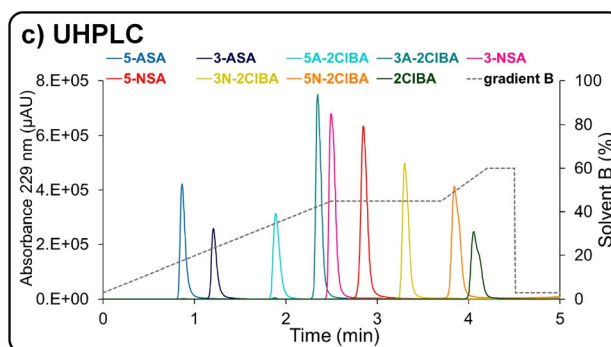
Figure 5. The reaction and analytics setup used for the hydrogenation. a) Detailed reaction setup schematic (P and T = pressure and temperature sensors). b) Representative infrared spectrum used for species quantification with a PLS model. The region considered is highlighted, with the insert showing the pretreated spectrum fed into the model. c) A demonstration of the species separation achieved in the developed online UHPLC method. The solvent gradient is plotted as a dotted line (gray). Note: an additional 2.5 min is allowed (not shown) for equilibration, prior to the next injection.
