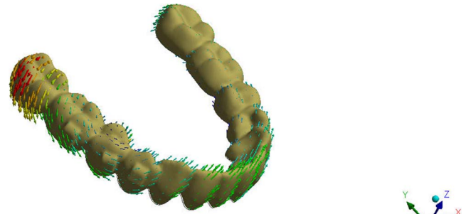
Figure 8. Aligner deformation of the ATT 4.4–4.6 3° simulation.
