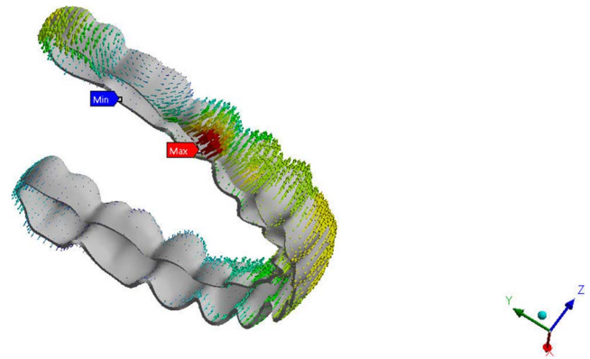
Figure 2. Aligner deformation of the NO ATT 1.2° simulation.
