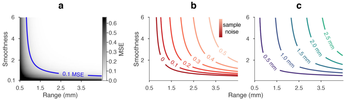
Figure 3. Effects of covariance model parameters on expected prediction loss. (a) Kriging MSE (eq 4) was calculated for 1 mm spacing, unit variance, and zero noise over a Matérn parameter space. MSE was monotonic in both range and smoothness parameters. Our threshold for predictability was 10% MSE relative to process variance (blue isocontour). Predictability was limited by a low value of either parameter. Smoothness had a weak influence on predictability when range was below a limit, and vice-versa. (Exact limits depended on the sampling geometry.) (b) The 10% predictability threshold for 1 mm grid pitch was computed under increasing levels of sample noise. In higher noise, predictability was restricted to smoother and longer range fields. (c) Predictability thresholds at 20% noise and varied grid pitch from 0.5 to 2.5 mm. Increasing or decreasing pitch had a similar effect on predictability as increasing or decreasing noise. By reducing pitch to 0.5 mm, approximately the same fields were predictable in 20% noise as were predictable in 0% noise and 1 mm pitch.
