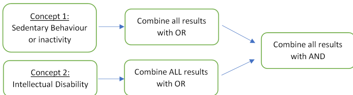
Figure 1. Search strategy.
