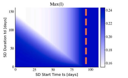
(b) Weighted average of periodic transmission rate combined with a single-pulse SD.
