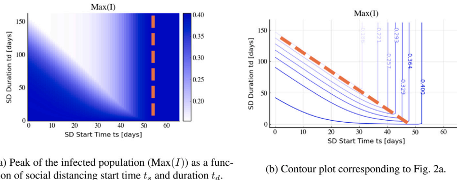
Fig. 2. Infected peak, \text{Max}(I) , under single interval social distancing (SD) policy. Time is measured in days, and the parameters used for the SIR model are \beta_n = 0.2 , \beta_d = 0.1 , and \gamma = 0.05 (see Eqs. (1) and (3)). (For interpretation of the references to color in this figure legend, the reader is referred to the web version of this article.)
