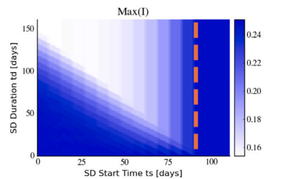
(d) Periodic relaxation with T = 7 and r = 5/7 combined with a single-pulse SD.
