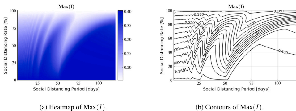
Fig. 7. Infected peak Max(I) of SIR model (1) under various periodic distancing policies with different period T and ratio of social distancing r . See Fig. 2 for parameter values.
