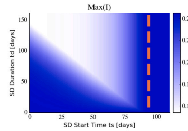
(c) Periodic SD with T = 1 and r = 5/7 combined with a single-pulse SD.
