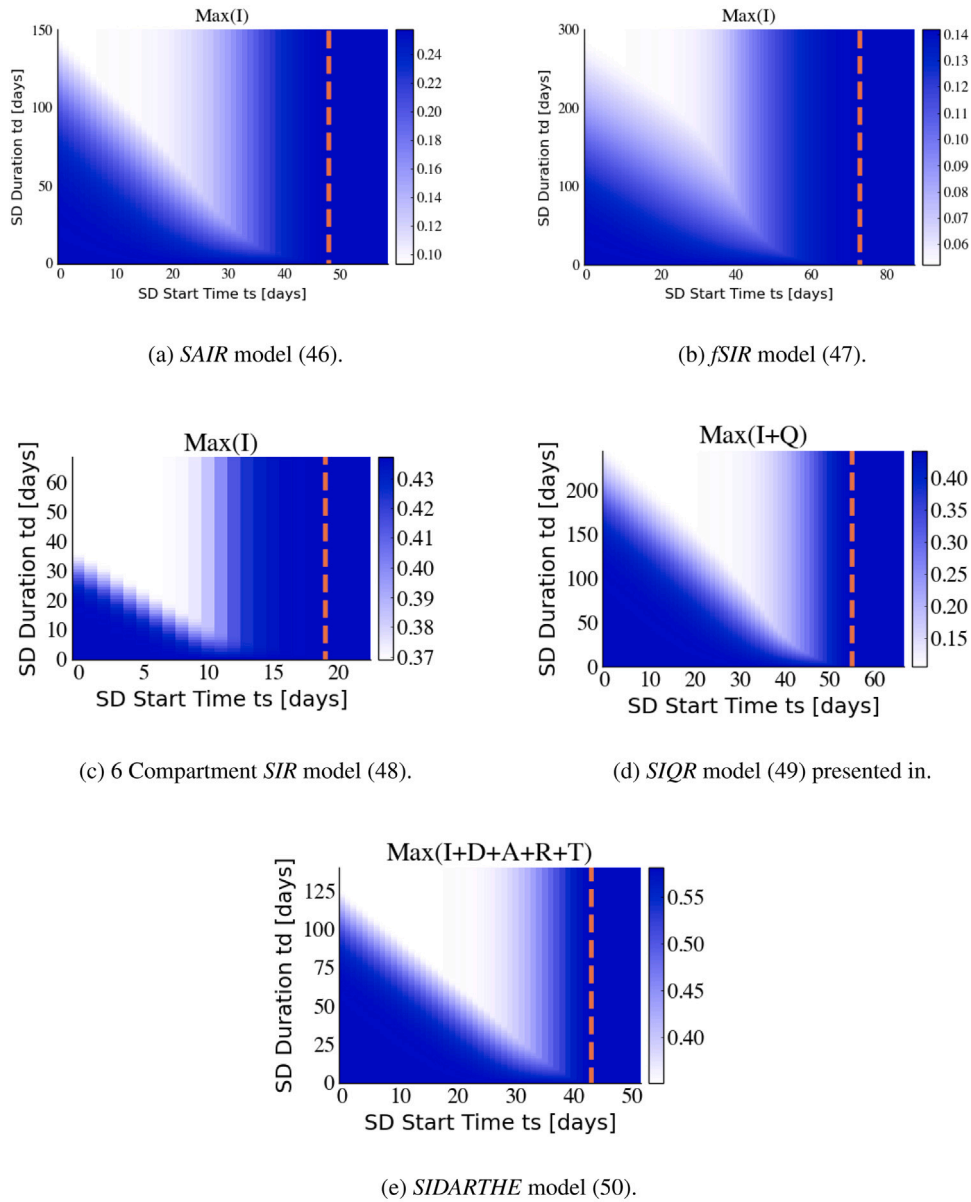
Fig. 6. Recent models proposed to capture the COVID-19 behavior show the “V” pattern. Models and their parameters are fully presented in Appendix C. The ratio between transmission rates of normal and socially distanced populations ( \beta_n/\beta_d ) is fixed at 2 for all models. (For interpretation of the references to color in this figure legend, the reader is referred to the web version of this article.)
