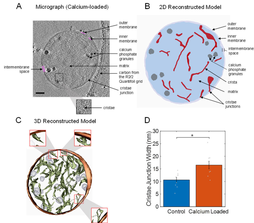
Figure 3. Calcium-loaded mitochondria with granules alters cristae structure. (A) Representative portion of a tomogram from a mitochondrion with calcium phosphate granules exposed to a 50 \mu\text{M} bolus of calcium at an approximate resolution of 4 \text{\AA} . The solid magenta lines highlight the inner or outer membrane boundaries. (B) 2D reconstructed model showing that calcium phosphate granules disrupted the cristae membrane surface area, consisting of most of the enzymes responsible for oxidative phosphorylation. (C) 3D reconstructed model showing a densely packed, interconnected cristae network. (D) Cristae junction widths in calcium-loaded mitochondria, which were significantly larger than the control widths. Approximately 10 cristae junctions from each type of mitochondrion were selected at random and measured. The bars are plotted as means of the data, with error bars representing the standard error of the mean. A * signifies a p value less than 0.01. Gray dots are individual data points. Scale bar = 250 nm.
