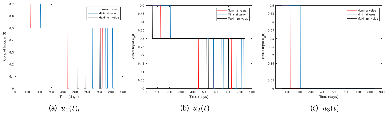
Fig. 11. Control inputs for Case 1, Model parameters with nominal, minimum, and maximum values.
