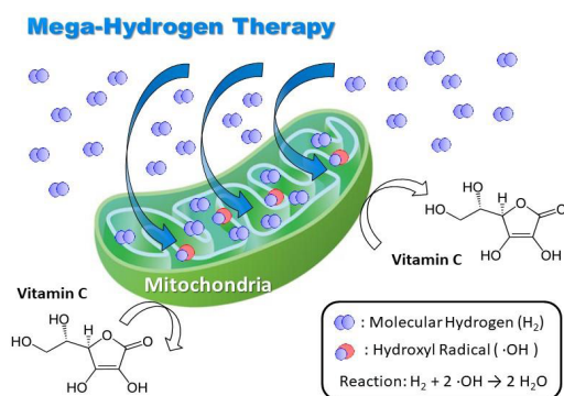
Figure 1: Large amounts of molecular hydrogen scavenge the hydroxyl radicals generated inside the mitochondria and improve disease.
