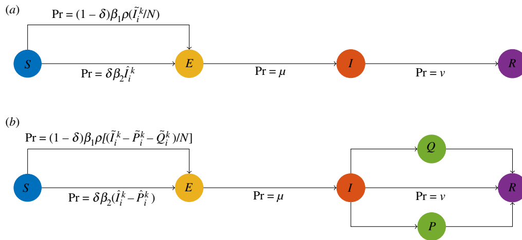
Figure 1. (a) The schematic diagram of the basic epidemiological model. (b) The schematic diagram of the adjusted epidemiological model with an isolation state, where P is the compartment of individuals practising separated isolation and Q is the compartment of individuals practising home isolation. The probabilities displayed in both diagrams are for each simulated individual.
