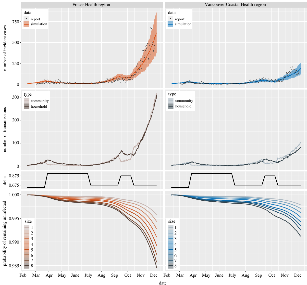
Figure 3. Top: the number of incident cases from simulation (mean curves with 10–90 percentile range bands) and reported data (points) in the two regions. Middle: the first row displays the number of community and household transmissions from simulations in the two regions; the second row depicts the values of parameter \delta described in table 2. Bottom: the survival curves for individuals in households of different sizes from simulations in the two regions. All curves in the figure reflect mean values over 100 runs for each of the simulations. Model parameters are the same in the two regions, except for the household size distribution.
