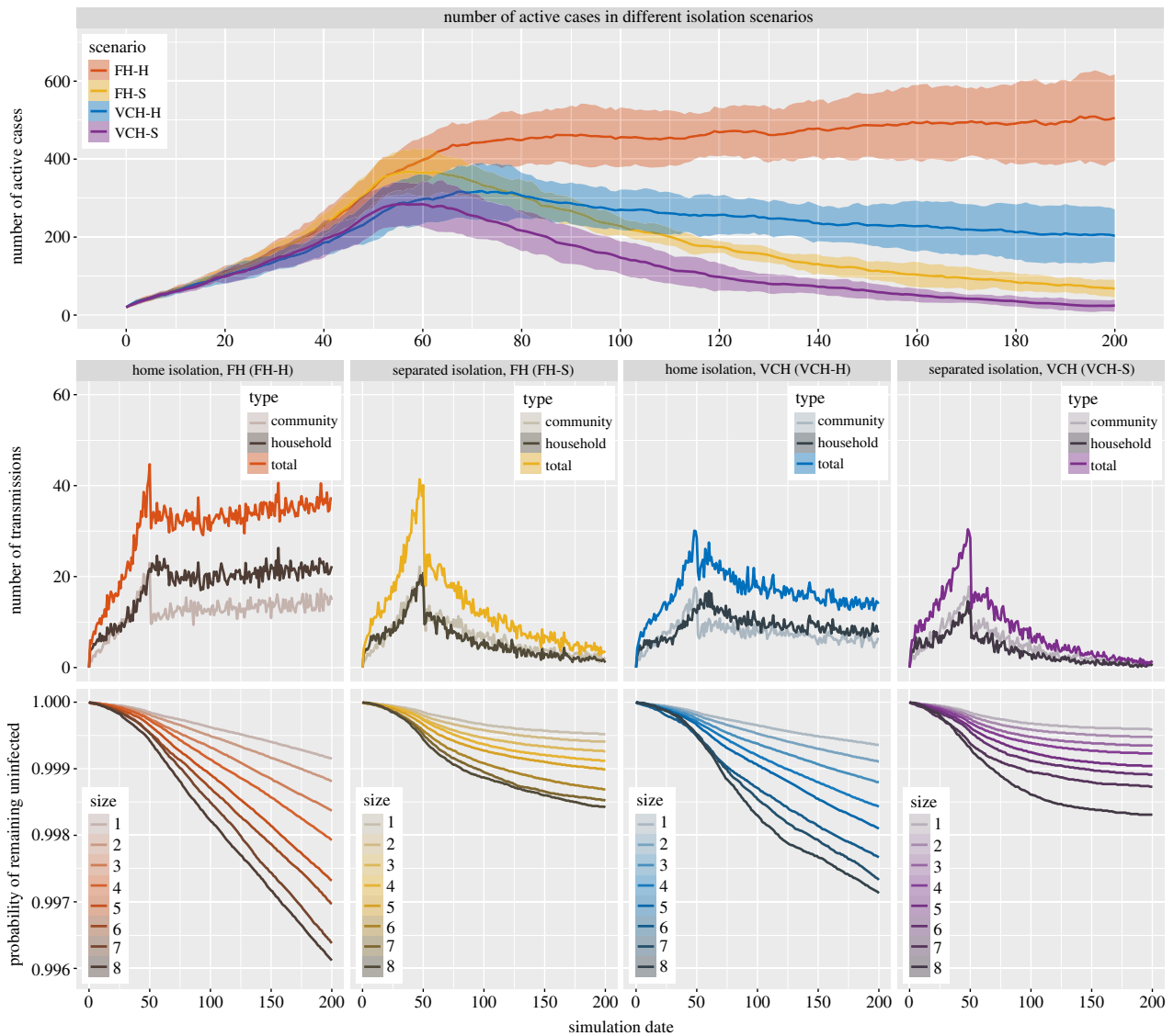
Figure 4. Results of simulations for isolation scenarios where 55% of the simulated individuals practise home or separated isolation. Top: the number of active cases (mean with 10–90 percentile range bands) in each of the isolation scenarios. Middle: the number of transmissions of different types in each of the isolation scenarios. Bottom: the survival curves for individuals in households of different sizes in each of the isolation scenarios. All curves in the figure reflect mean values over 100 runs of the simulation for each of the isolation scenarios and the settings only differ in household size distribution and the individuals' isolation preferences. The curves are organized so that warm colours (red and yellow) represent scenarios in FH and cold colours (blue and purple) represent scenarios in VCH.
