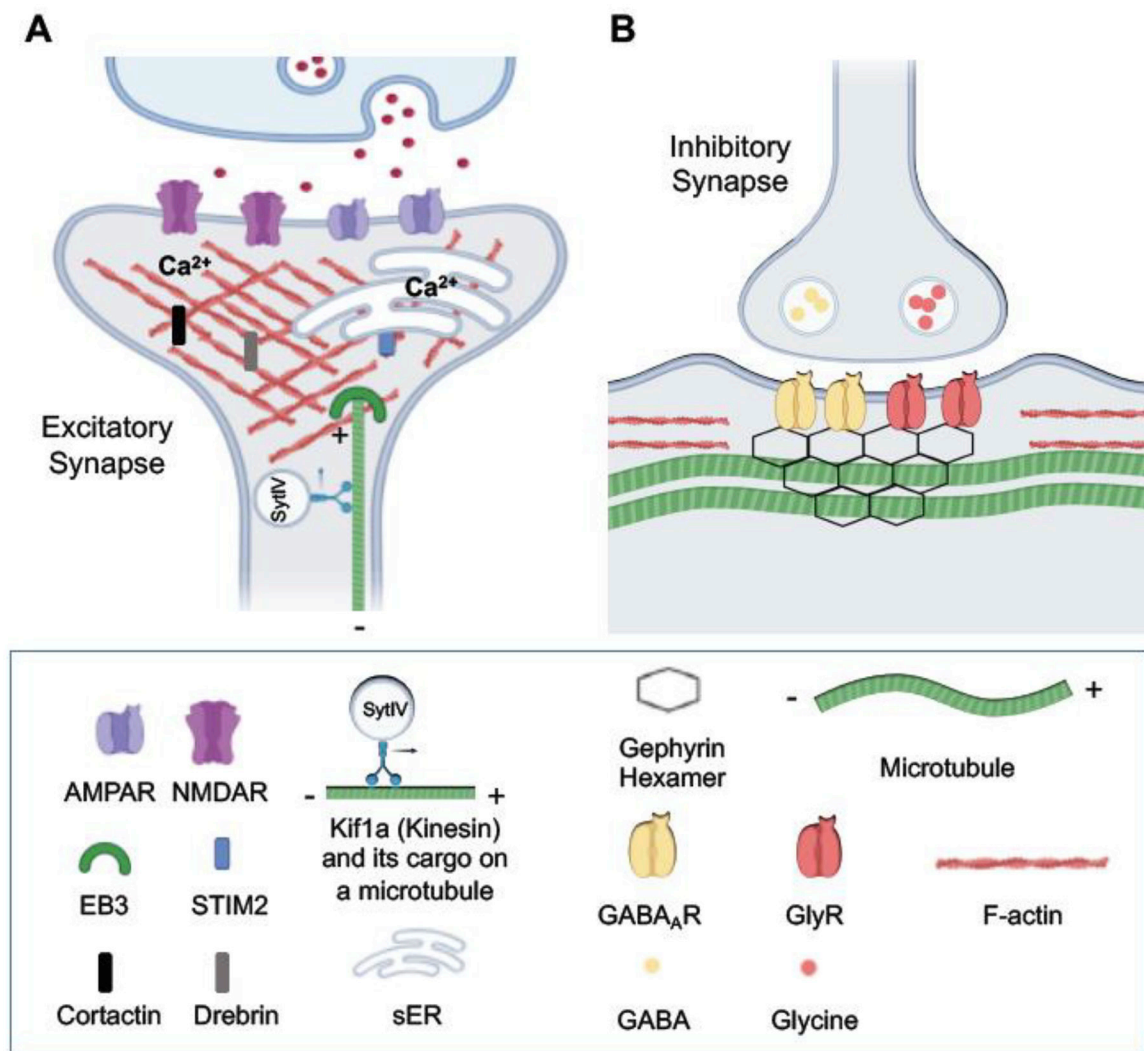
Figure 1. Schematic of MT functions in two different types of postsynaptic elements.
