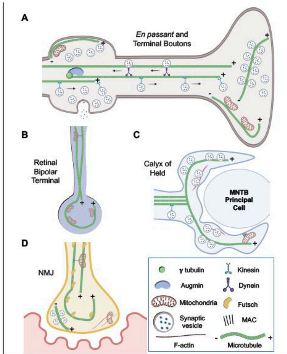
Figure 2. Schematic of MT functions in different types of presynaptic elements.
