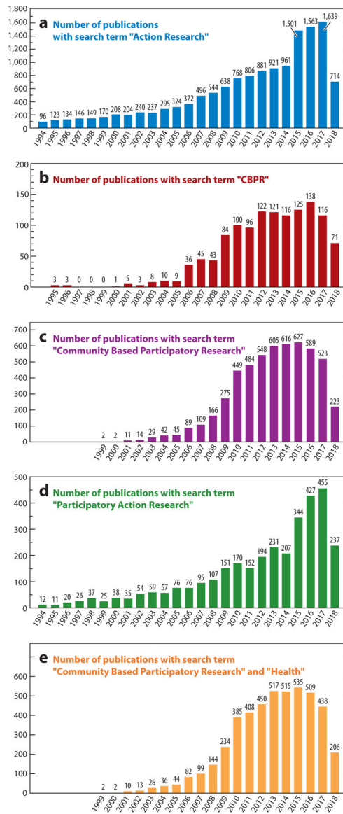
Figure 2. Charts displaying frequency of publications with key search terms.
