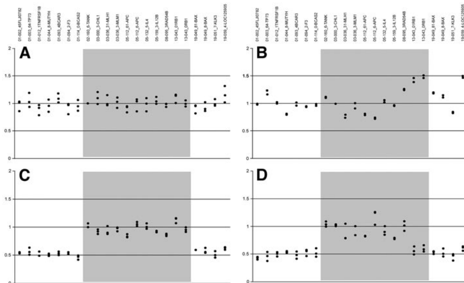
Figure 3. Representative scatterplots of normalized peak heights. Each plot represents one sample from one experiment with electroforesis in duplicate or triplicate. On the left in white 1p, on the right in white 19q, in grey the reference probes. A. Non-neoplastic brain tissue. B. Oligodendroglioma with FISH 0.99 for 1p and FISH 0.95 for 19q. C. Oligodendroglioma with FISH 0.59 for 1p and FISH 0.57 for 19q. D. Oligodendroglioma with FISH 0.54 for 1p and FISH 0.58 for 19q.
