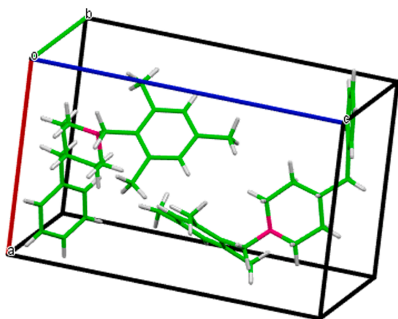
Fig. 2. Unit cell packing arrangement viewed through crystallographic axis a^*
