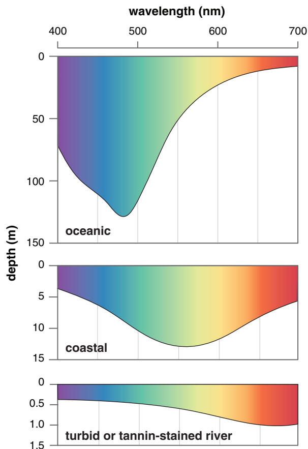
Fig. 1. Schematic of underwater light environments. Data adapted from Jerlov (1968) and Costa et al. (2013).
