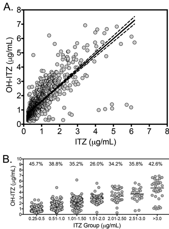
FIG 1 (A) Linear regression analysis between ITZ and OH-ITZ. ITZ and OH-ITZ were measured by validated HPLC or UPLC-MS assays, and concentrations within the analytical measurement range (0.25 to 6 \mu\text{g/ml} ) were plotted ( n=1,223 ). (B) OH-ITZ concentrations based on different ITZ concentration levels. The percent coefficients of variation of OH-ITZ are presented above each ITZ group.
