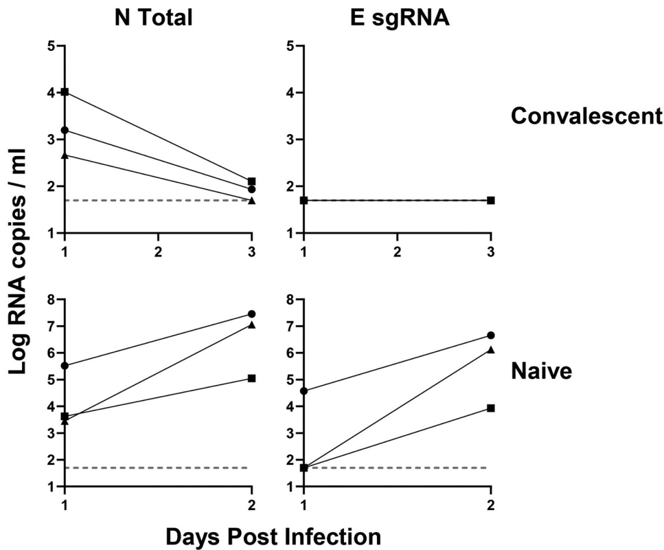
FIG 6 Convalescent NHP SARS-CoV-2 RT-PCR. NHPs were challenged with SARS-CoV-2 and rechallenged 35 days later. RNA extracted from nasal swabs from the rechallenge macaques was run for N total and E sgRNA in naive and the same convalescent animals.
