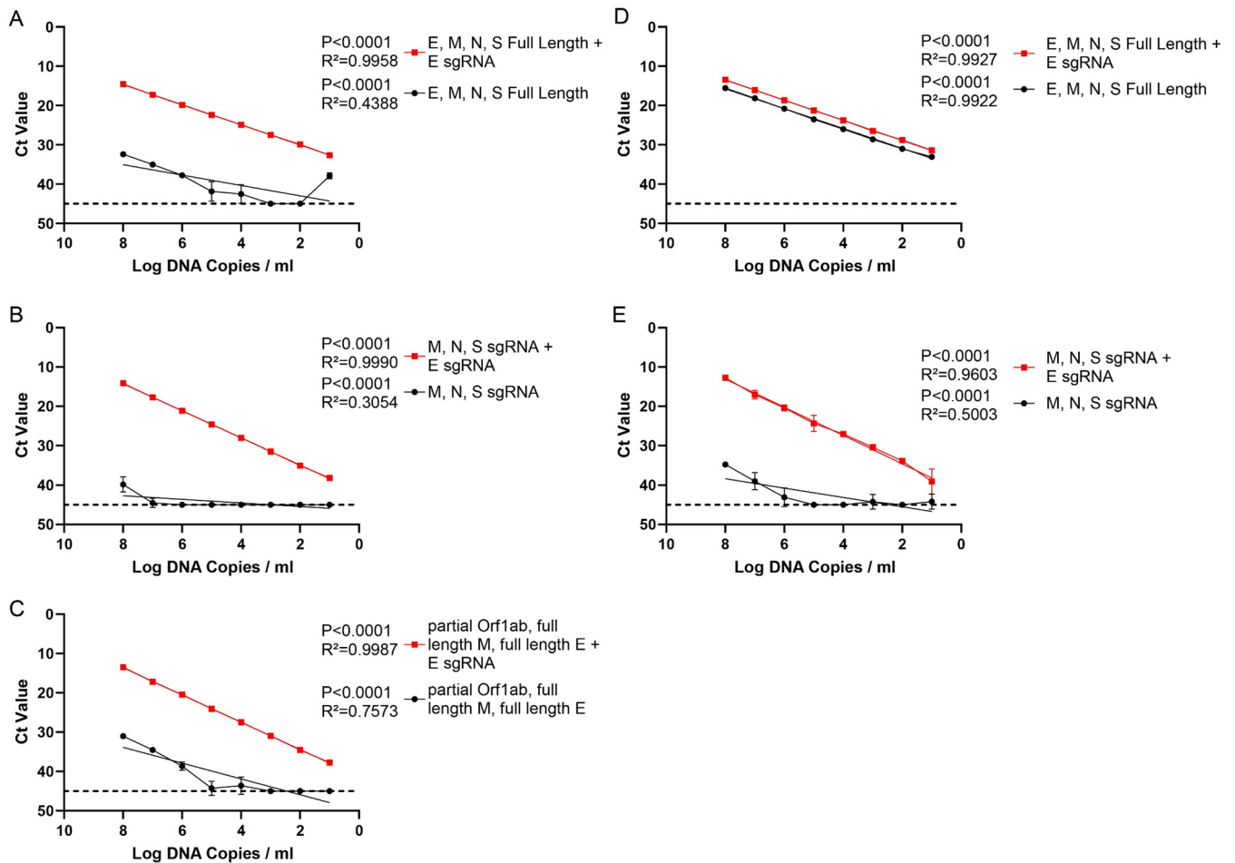
FIG 3 Assay specificity with linear DNA mixtures. RT-PCR was performed on DNA fragment mixtures with and without the addition of E sgRNA linear DNA fragments. These mixtures were serially diluted 10-fold from 10^8 to 10 copies per ml. (A) Mixture of E, M, N, and S full-length DNA fragments. (B) Mixture of M, N, and S subgenomic partial DNA fragments. (C) Mixture of E and M full-length DNA fragments and the 5' end of Orf1a containing the subgenomic leader sequence. In all mixtures, linearity was only present after the addition of E sgRNA. RT-PCR targeting E gRNA was performed on DNA fragment mixtures with and without the addition of an E sgRNA DNA fragment. (D) Mixture of E, M, N, and S full-length DNA fragments. (E) Mixture of M, N, and S subgenomic DNA fragments. Error bars denote the 95% confidence intervals of the mean of eight technical replicates. Lines represent simple linear regressions.
