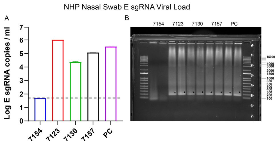
FIG 2 SARS-CoV-2-infected NHPs were sampled through nasal swabs on day 4 postinfection. (A) RNA was extracted from the nasal swabs and an E sgRNA RT-PCR assay was performed. (B) The assay RT-PCR results were then run in duplicate on a 0.8% agarose gel to confirm a single amplicon. Error bars define the standard deviation of the mean of two technical replicates for each macaque. PC indicates positive control. Asterisk indicates expected band.
