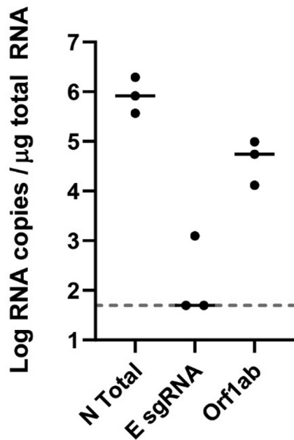
FIG 4 Infectious cell lysate treated with RNase A. Infectious cell lysate was treated with RNase A for 1 h and then RNA was extracted and RT-PCR for the N gene (N total), subgenomic E (E sgRNA), and genomic RNA (Orf1ab) was performed. Black bars represent median responses.
