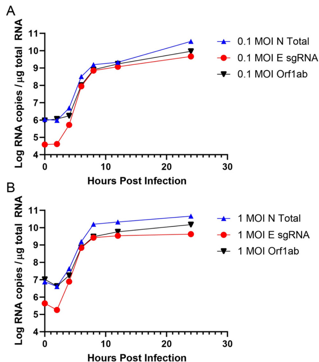
FIG 5 Longitudinal SARS-CoV-2 infection. Vero-E6 cells were infected at 0.1 MOI (A) or 1.0 MOI (B) in 12-well plates. Wells were harvested in triplicate at the following time points: 0, 2, 4, 6, 8, 12, and 24 h postinfection.
