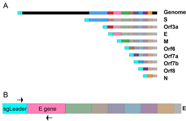
FIG 1 Graphical representation of sgRNAs and the E sgRNA assay. (A) Graphical representation of SARS-CoV-2 virus and sgRNA. Upon cellular entry SARS-CoV-2 generates sgRNAs for structural genes and accessory proteins before they are produced. The subgenomic leader sequence is colored cyan to highlight its position in the genomic and subgenomic RNAs. (B) Graphical representation of the primer binding sites for the E sgRNA assay on subgenomic E RNA. The forward primer binds to the subgenomic leader sequence present on all subgenomic RNAs as well as the genomic RNA. The reverse primer binds to the E gene (pink).
