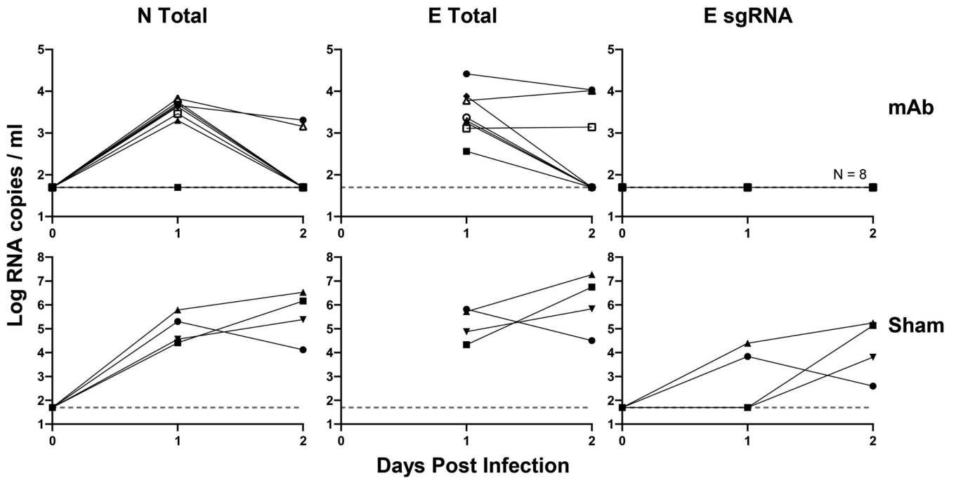
FIG 7 RT-PCR of mono-clonal antibody-protected NHPs challenged with SARS-CoV-2. NHPs were given 50 mg/kg of a mono-clonal SARS-CoV-2 antibody and then challenged 3 days later with SARS-CoV-2. RNA extracted by BAL fluid was measured for N total, E total, and E sgRNA. Protected macaques (MAb) were compared to unprotected macaques (sham) to demonstrate assay success.
